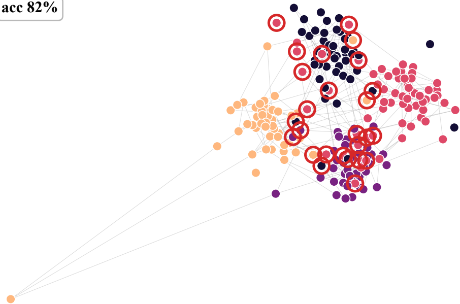
(b) learnable-Tsallis GNN ( \eta = 0.4 )
