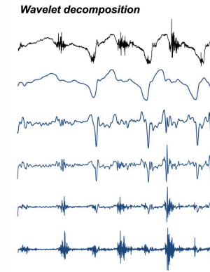
Figure 2. 5 level wavelet decomposition of hull acceleration signal.
