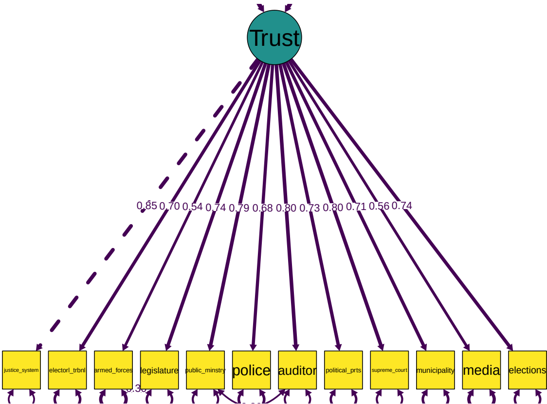
Figure A1 CFA Path Diagram for LAPOP Mexico Trust Scale (Fold 1 Training). Standardized loadings on paths; freed residual covariances between public ministry and auditor.
