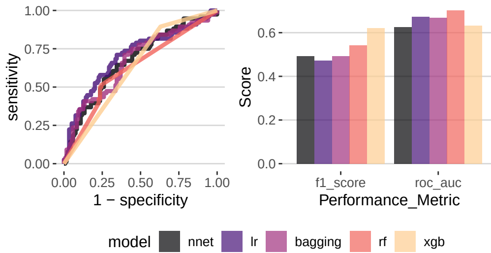
Figure 4. Final Model Selection Predicting Target Variable in Test Set.
