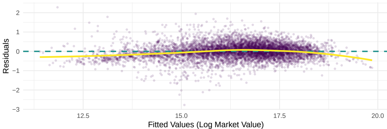
C. Residuals vs. Fitted Values
