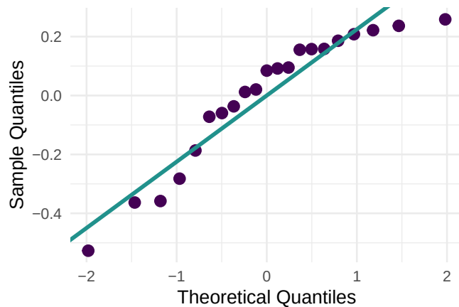
B. Club Random Intercepts (n = 21)
