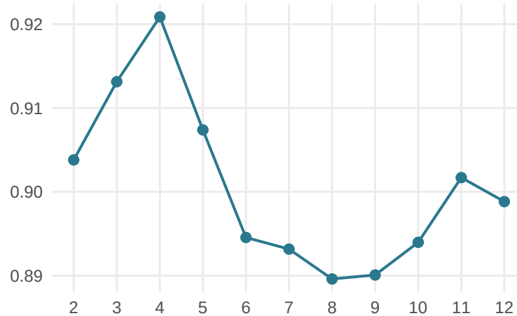
Classification sharpness
