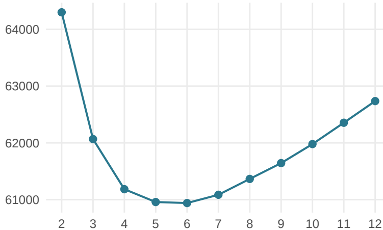
Weighted BIC (lower is better)
