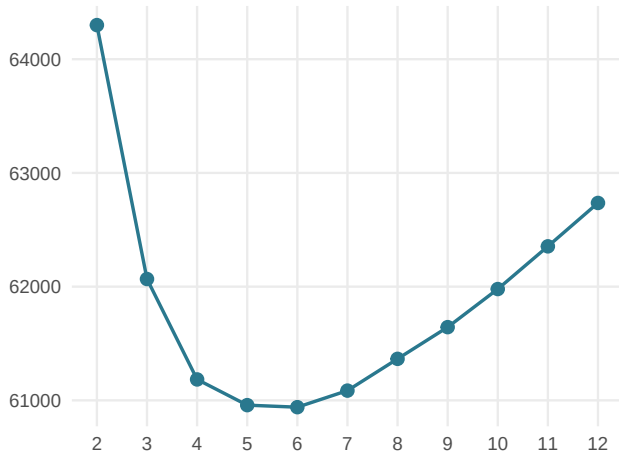
Weighted BIC
