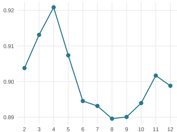
Relative entropy
