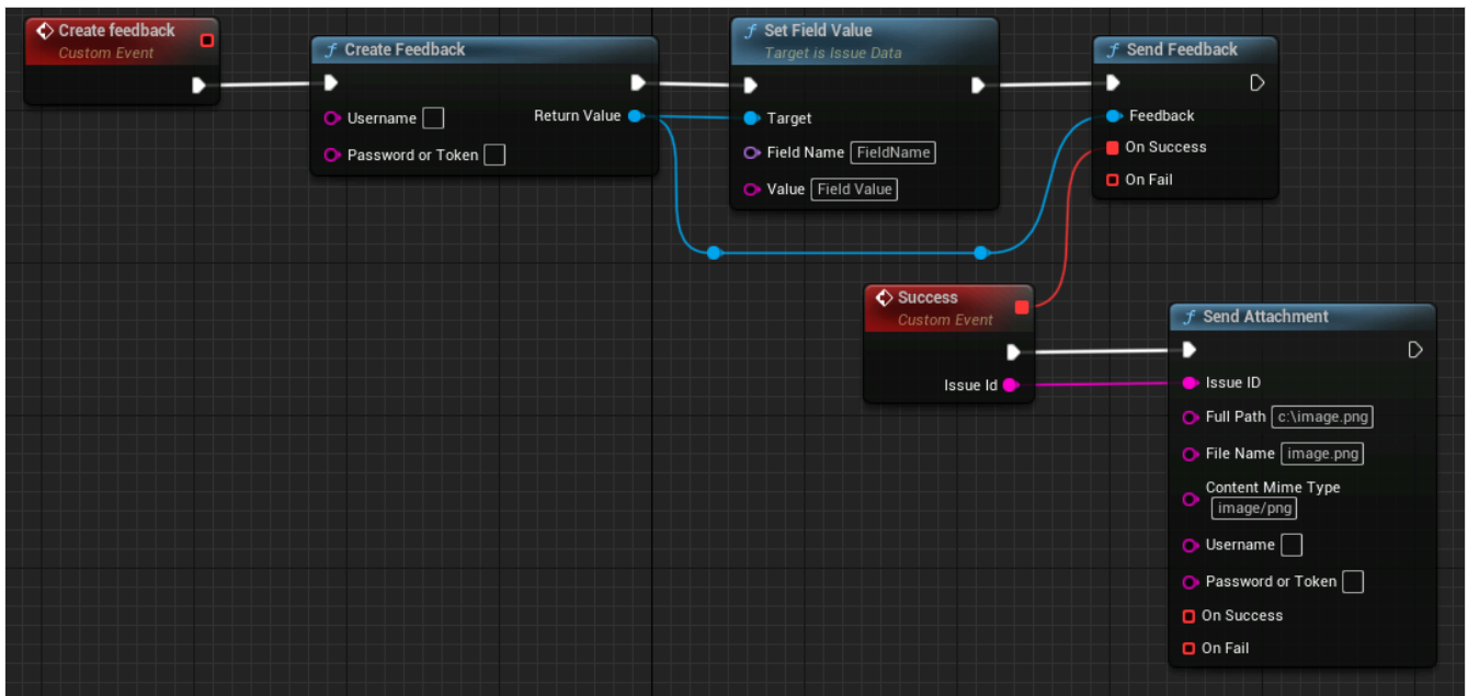
Example 5 - Send user feedback with attachment (async version)
