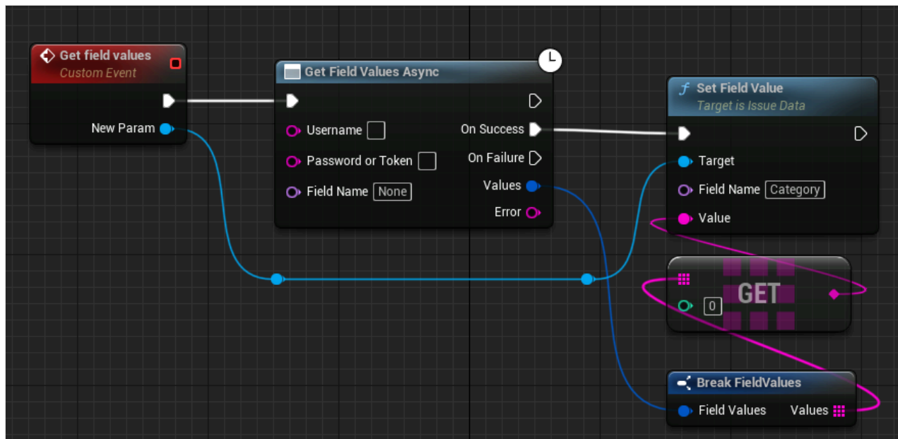
Example 6 - Get field values
