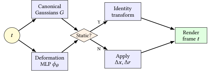
Figure 3: Canonical + deformation data flow (the canonical 4DGS route). At each frame t , the canonical Gaussians G and the shared deformation MLP \phi_\theta jointly decide whether each Gaussian is static (identity transform, no deformation) or dynamic (apply \Delta x, \Delta r ). Static Gaussians are rendered from a shared buffer (cacheable); dynamic Gaussians are rendered with per-frame deformation. This is the basis for the dynamic / static separation route explored in §3.2 and §4.1.
