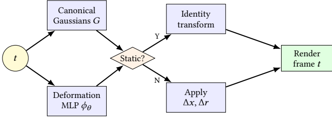
Figure 3: Canonical + deformation data flow (the canonical 4DGS route). At each frame t , the canonical Gaussians G and the shared deformation MLP \phi_\theta jointly decide whether each Gaussian is static (identity transform, no deformation) or dynamic (apply \Delta x, \Delta r ). Static Gaussians are rendered from a shared buffer (cacheable); dynamic Gaussians are rendered with per-frame deformation. This is the basis for the dynamic / static separation route explored in §3.2 and §4.1.
