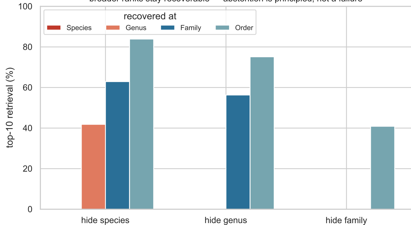
Missing-reference stress test (Eval C): the hidden rank collapses to 0, broader ranks stay recoverable — abstention is principled, not a failure
