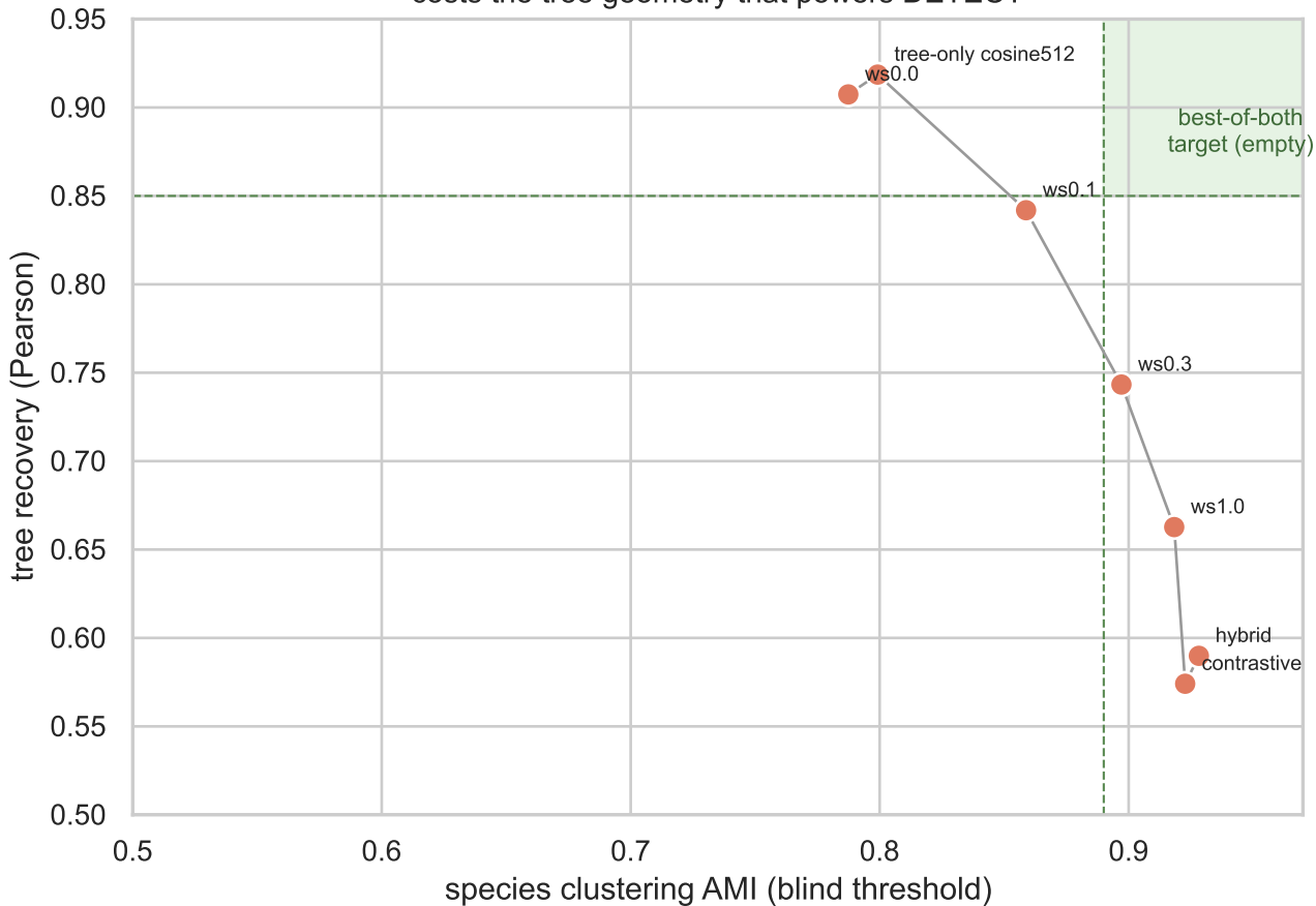
Tree-vs-species frontier: matching VSEARCH at species costs the tree geometry that powers DETECT
