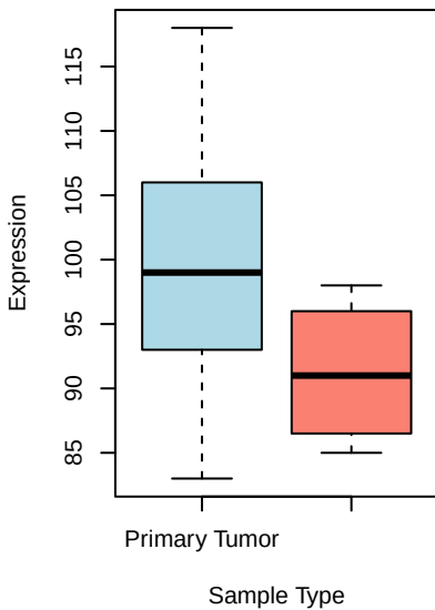
GENE_9
