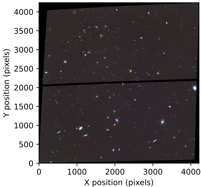
Hubble Ultra Deep Field
