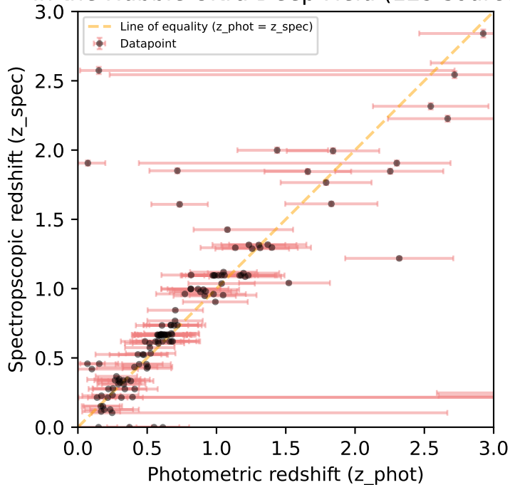
Photometric vs. Spectroscopic Redshifts in the Hubble Ultra Deep Field (129 sources)
