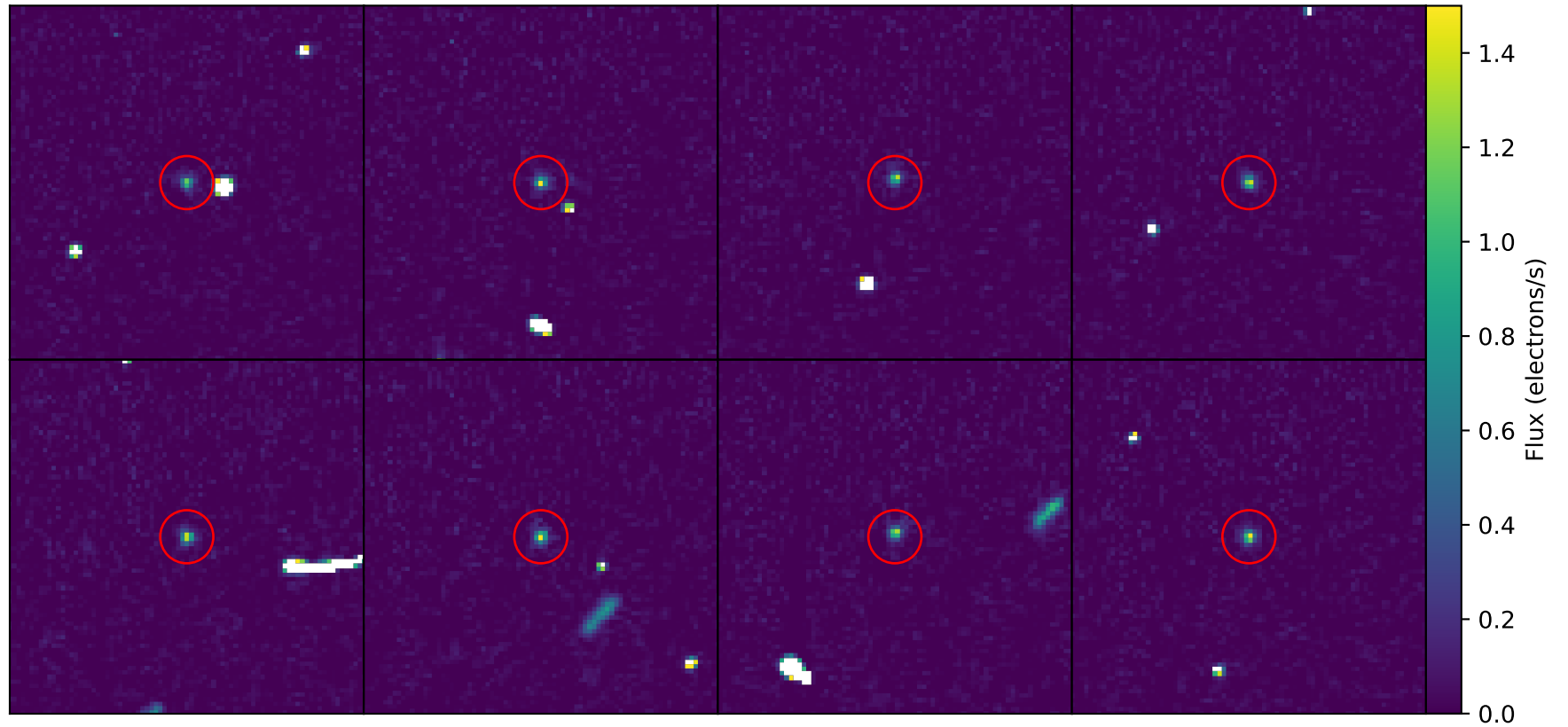
Kallichore 2025-Nov-30 HST/WFC3 image cutouts
