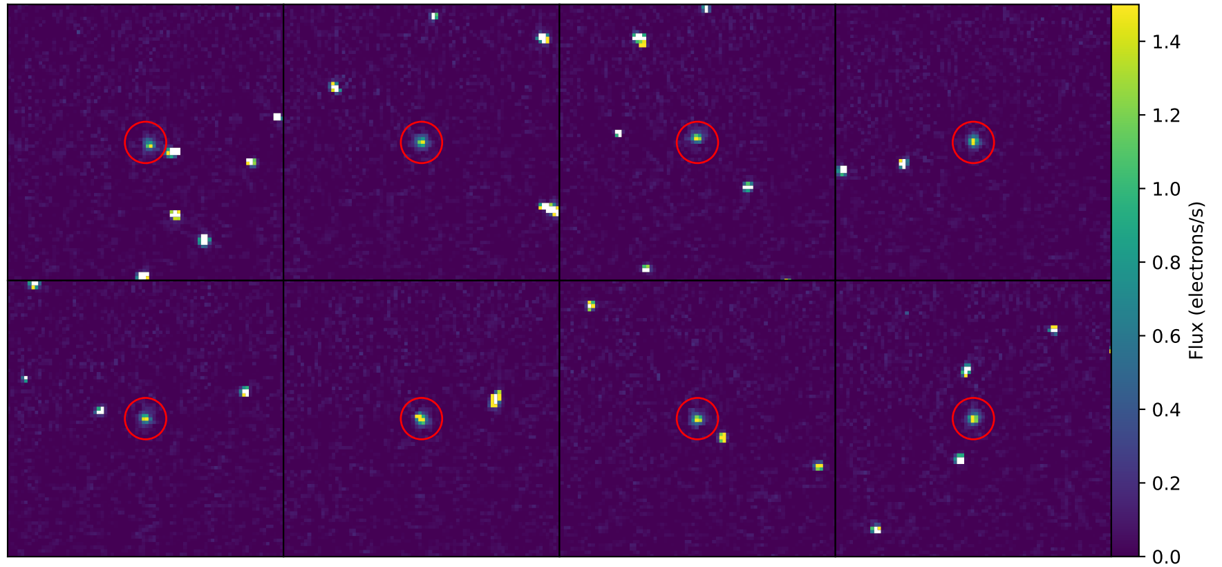
Kallichore 2025-Dec-05 HST/WFC3 image cutouts
