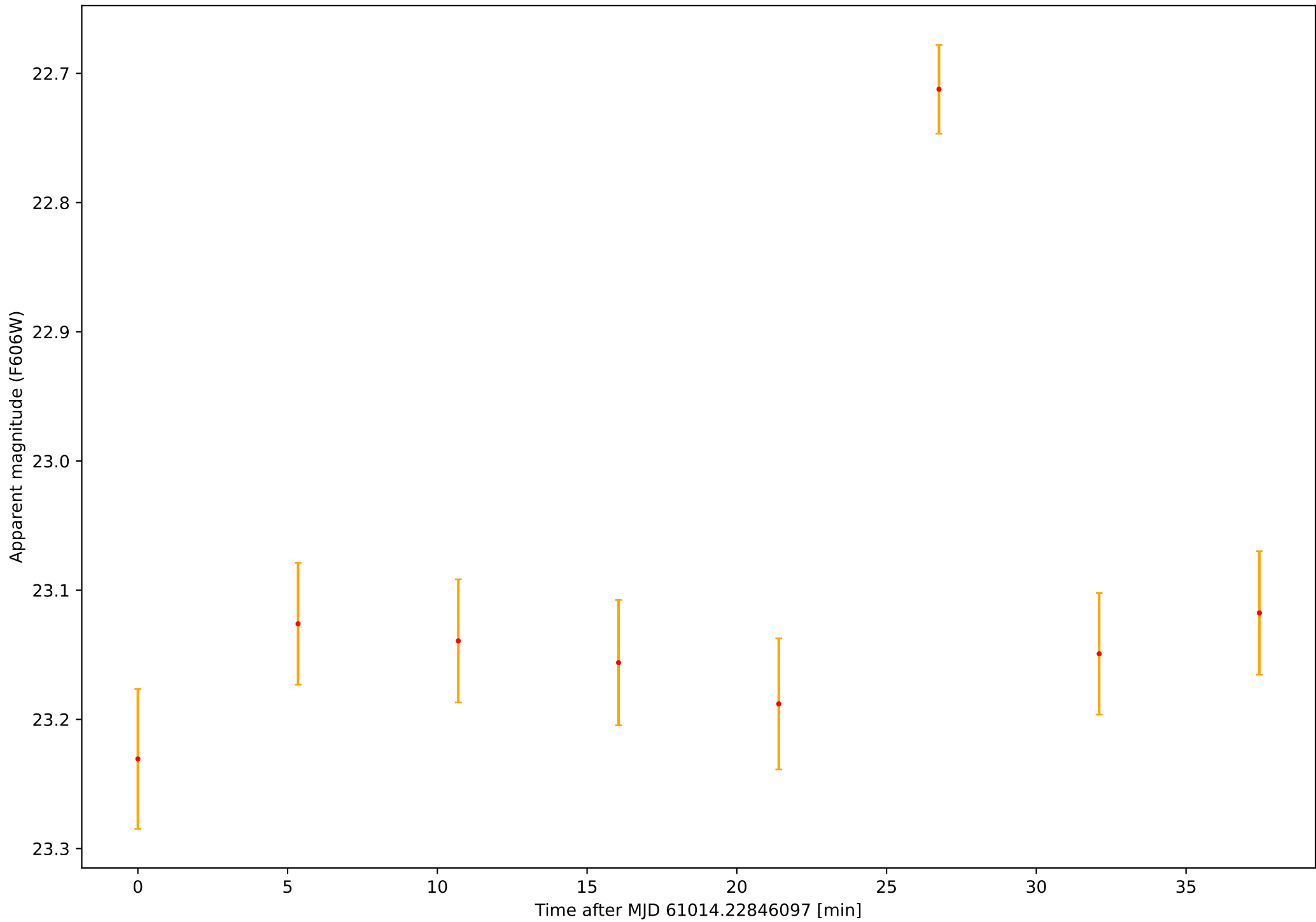
Kallichore F606W Lightcurve (2025-Dec-05)
