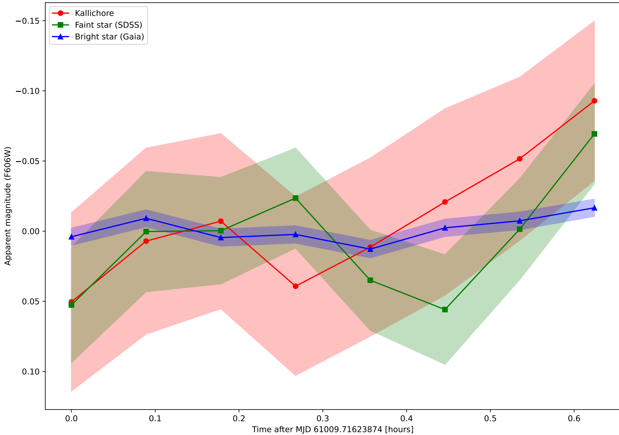
F606W Mag Variations (2025-Nov-30)
