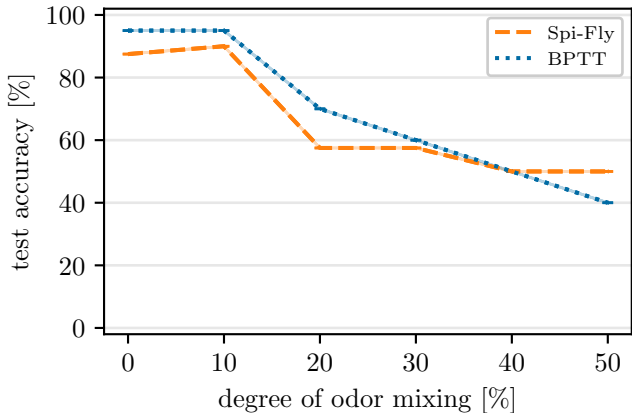
Vergara et al. gas sensor dataset
