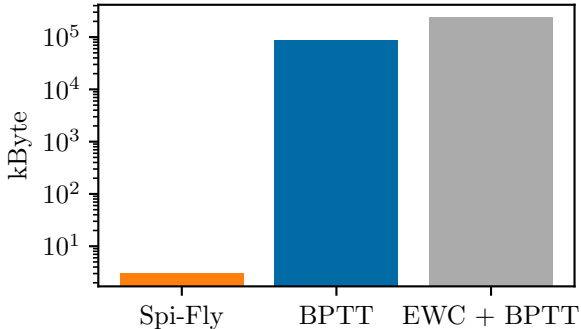
Off-chip memory required for learning
