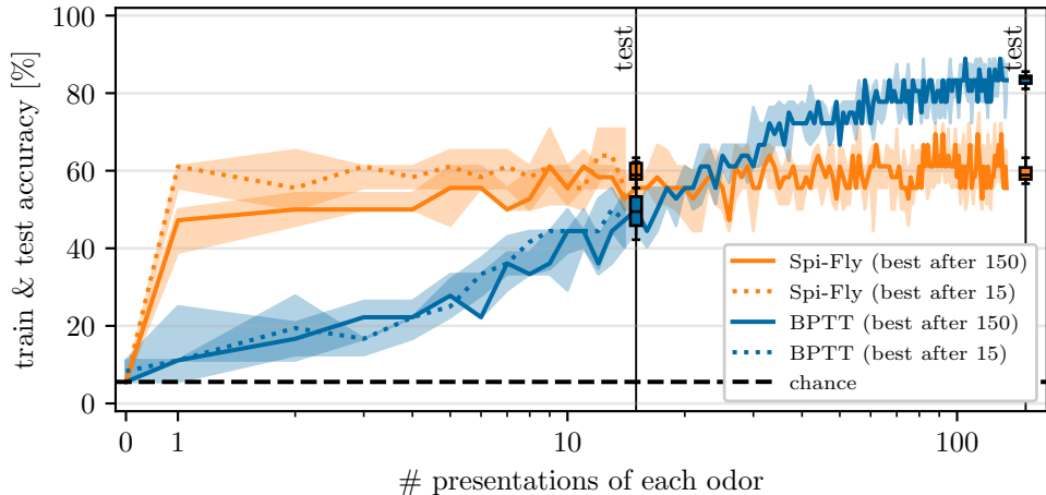
Synthetic DM responses (5 ORs, 18 odors)
