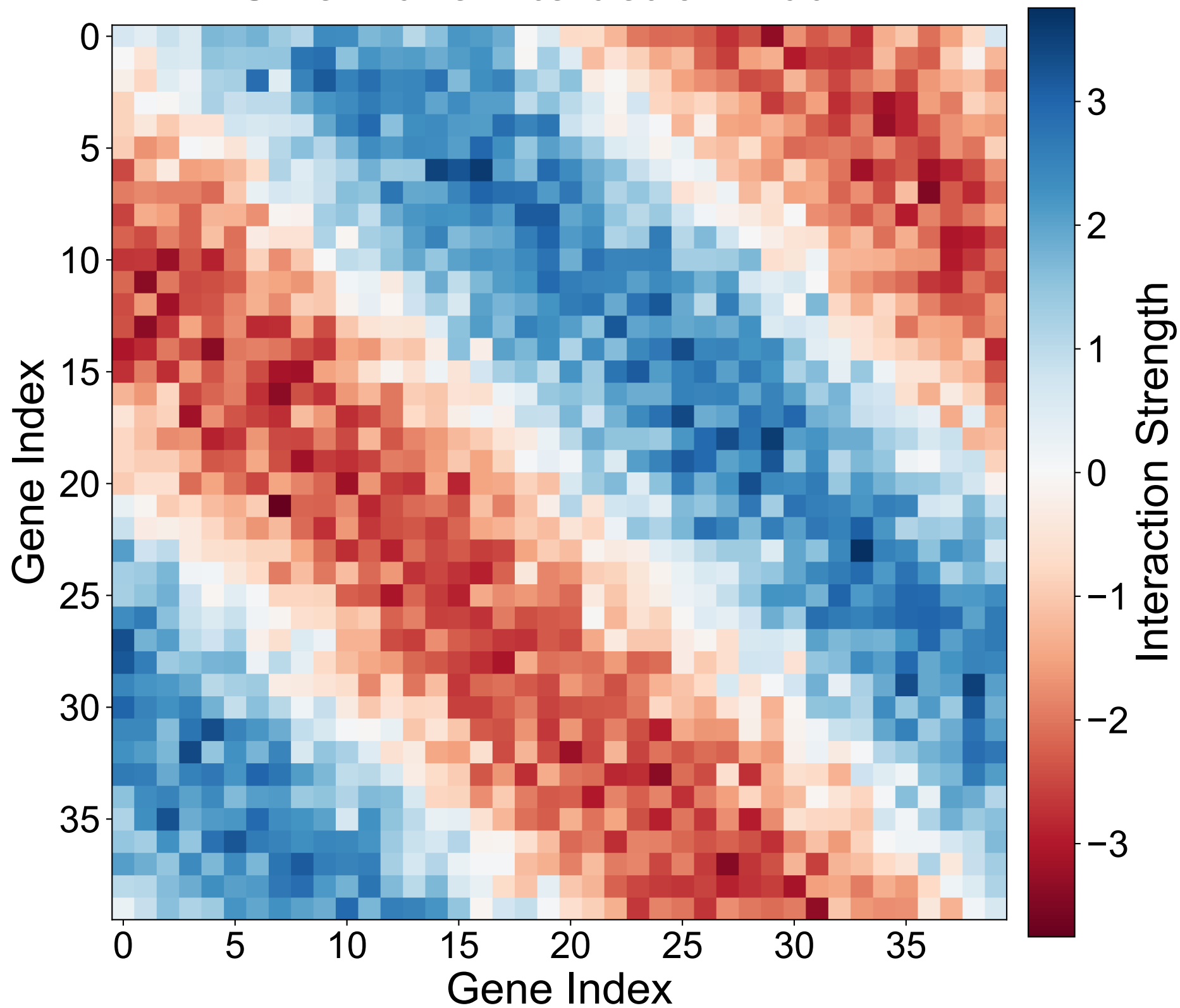
Sine Wave Interaction Matrix
