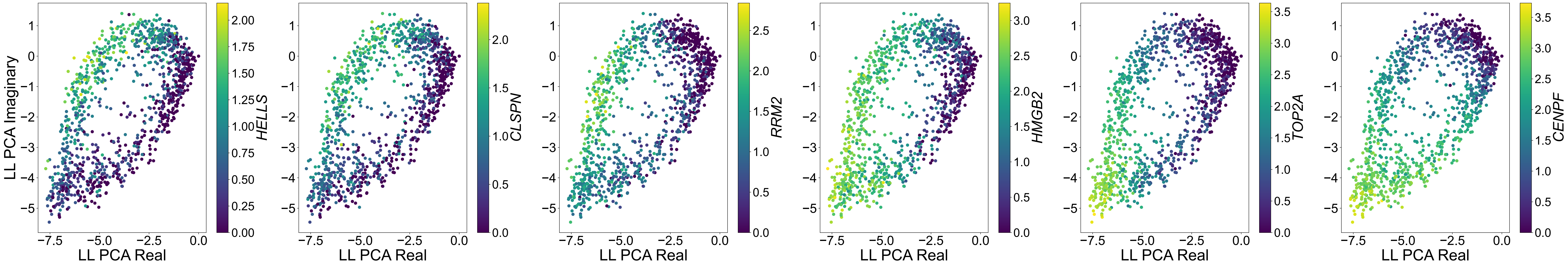
S Phase HELLS CLSPN RRM2 HMGB2 Phase = 2.20 rad, Amp = 0.17 Phase = 2.30 rad, Amp = 0.17 Phase = 2.92 rad, Amp = 0.16 Phase = 2.91 rad, Amp = 0.23 G2/M Phase TOP2A CENPF Phase = 3.28 rad, Amp = 0.22 Phase = 4.48 rad, Amp = 0.22
