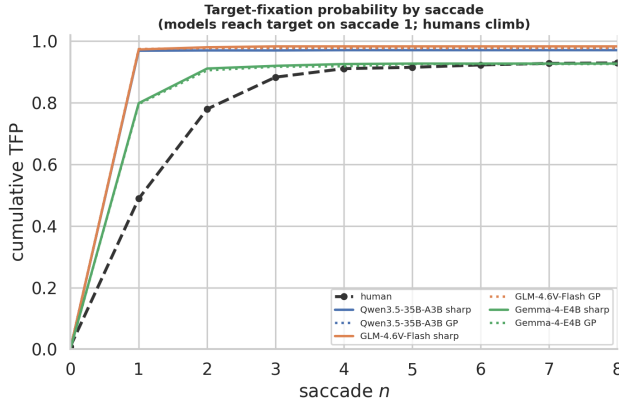
Fig. S2: Cumulative target-fixation probability by saccade (Eq. (3)) under SHARP (solid) and the human-matched GP (dotted) for the three models, against humans (dashed). The models reach the target on the first saccade; human probability accrues over several fixations.
