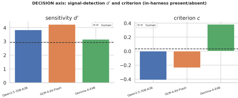
Fig. S1: Signal-detection sensitivity ( d' ) and criterion ( c ) for the in-harness present/absent decision, per model against the human reference.
