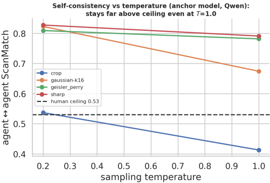
Fig. S10: Cross-seed self-consistency as a function of sampling temperature (anchor model, Qwen, core conditions), against the human↔human ceiling 0.53.
