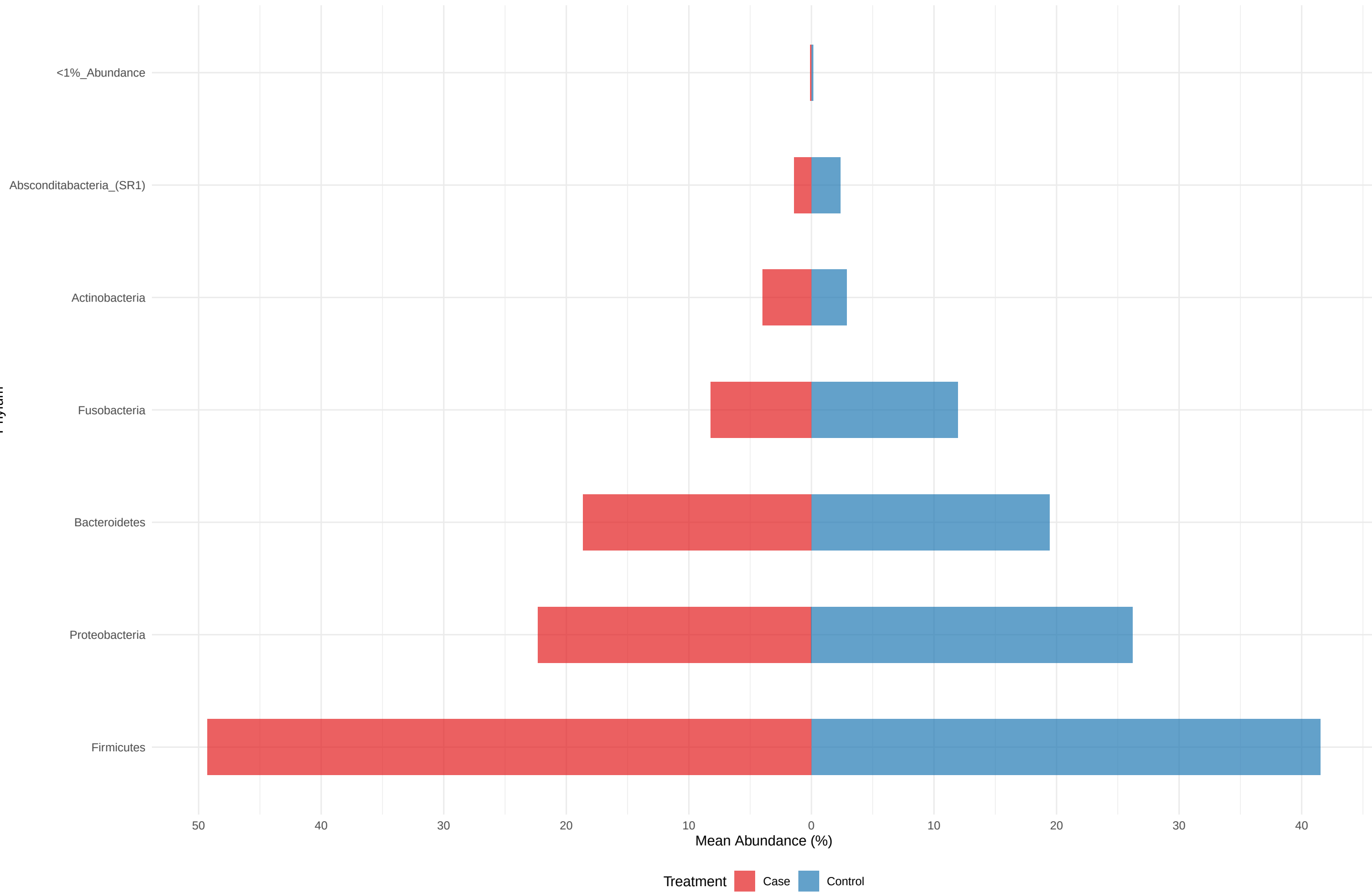
Bidirectional Plot of Phylum : Case vs Control
