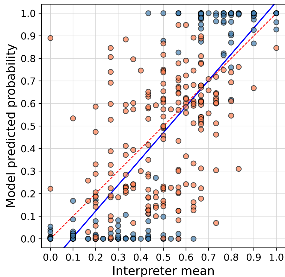
Random-forest stacking, no feature pass-through
