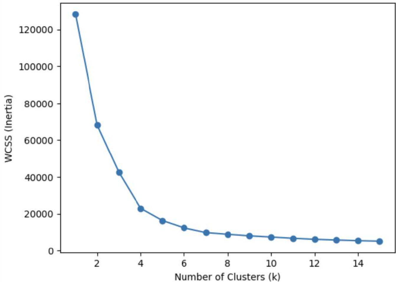
Elbow Method
