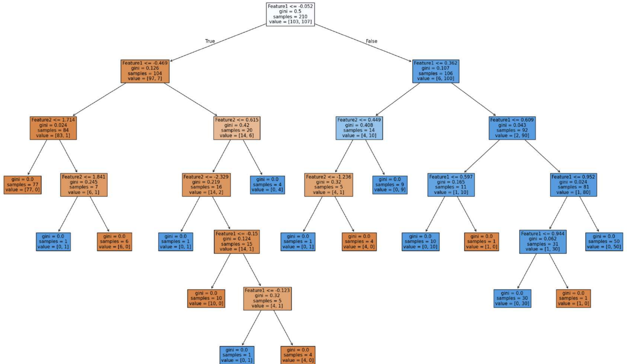
Fully Grown Classification Tree
