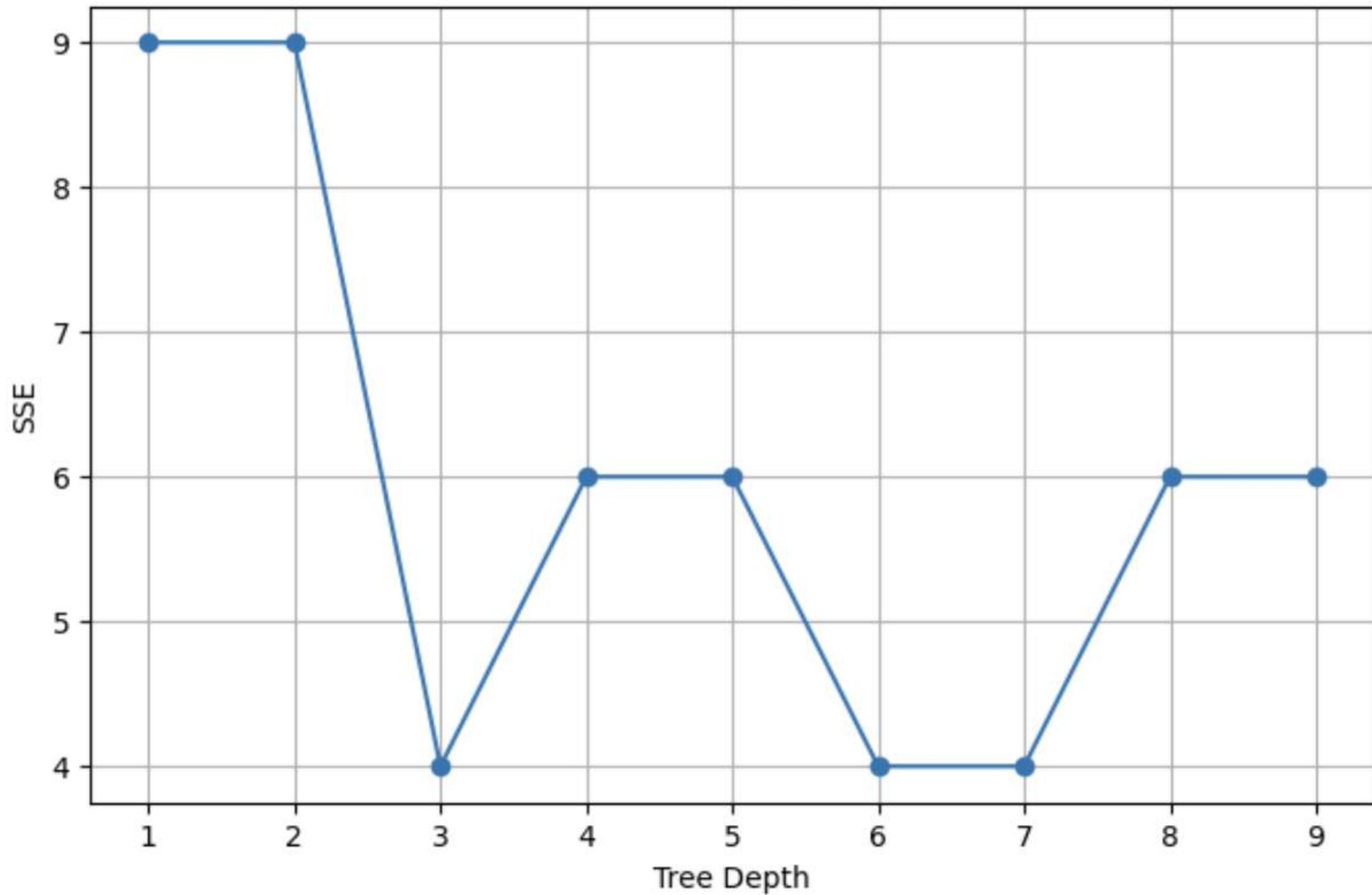
SSE vs Depth
