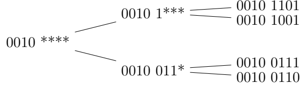
Figure 3: Patricia trie after adding 0010 0110 into the trie of Fig. 2
