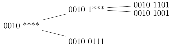
Figure 2: Example of Patricia trie
