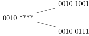
Figure 4: Patricia trie after deleting 0010 1101 from the trie of Fig. 2
