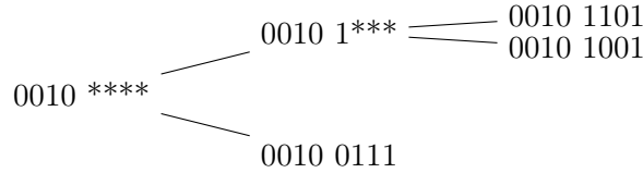
Figure 2: Example of Patricia trie
