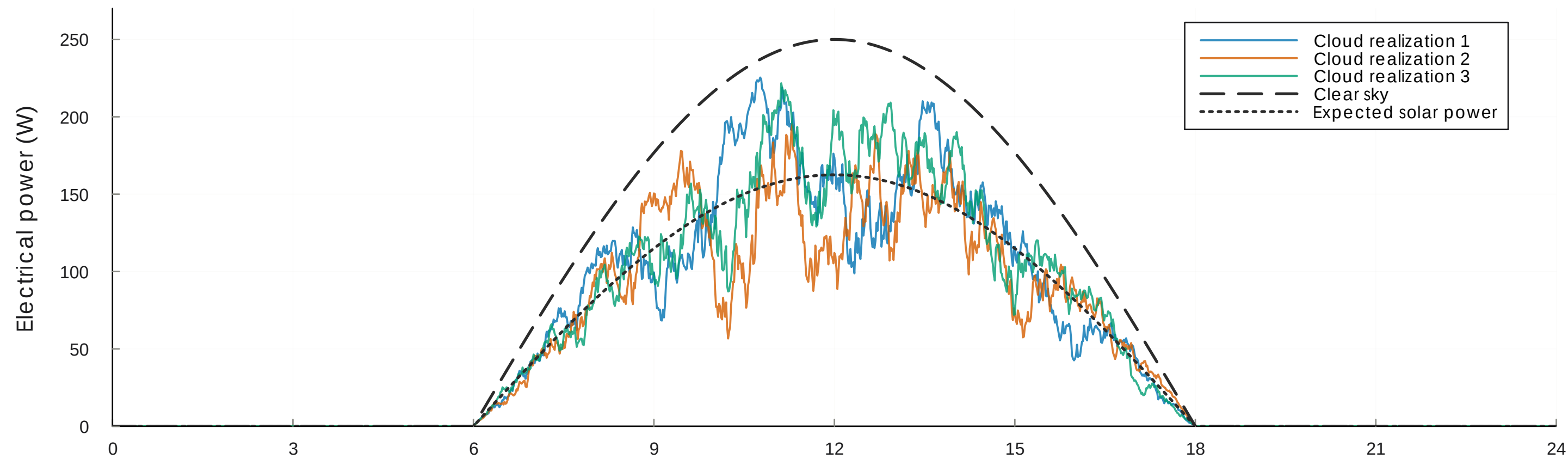
Solar power profile
