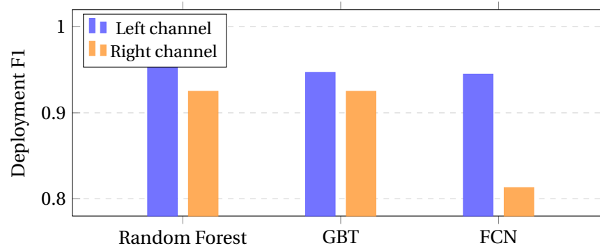
Figure 6.4: Deployment F1 by architecture and button channel on the held-out test set. The RF achieves the highest left-channel score (0.967); the FCN degrades substantially on the right channel (0.813) due to the smaller right-button corpus.
