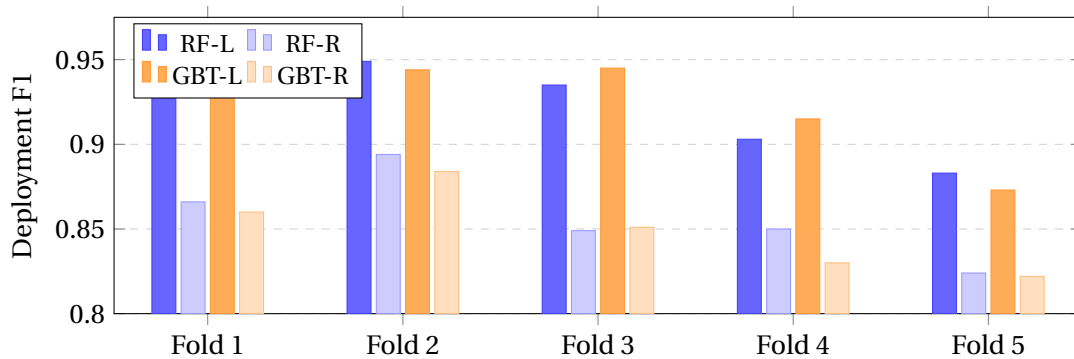
Figure 6.5: Per-fold LOPO deployment F1 for the four tree-based model variants. Fold 5 is consistently the lowest across all models, suggesting the held-out participant group in that fold has an atypically challenging click profile. The L-channel models outperform their R-channel counterparts in every fold, reflecting the larger left-button training corpus.
