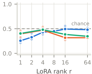
Unseen: A/B accuracy
