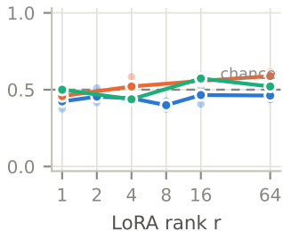
Seen: A/B accuracy
