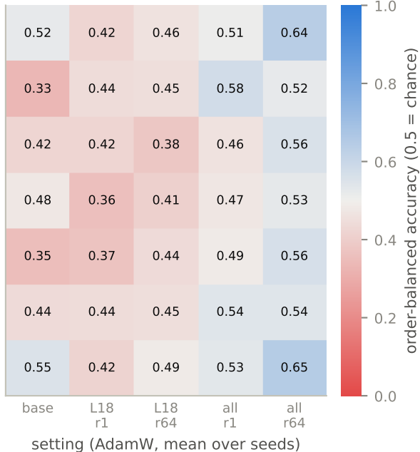
Seen presidents: A/B accuracy
