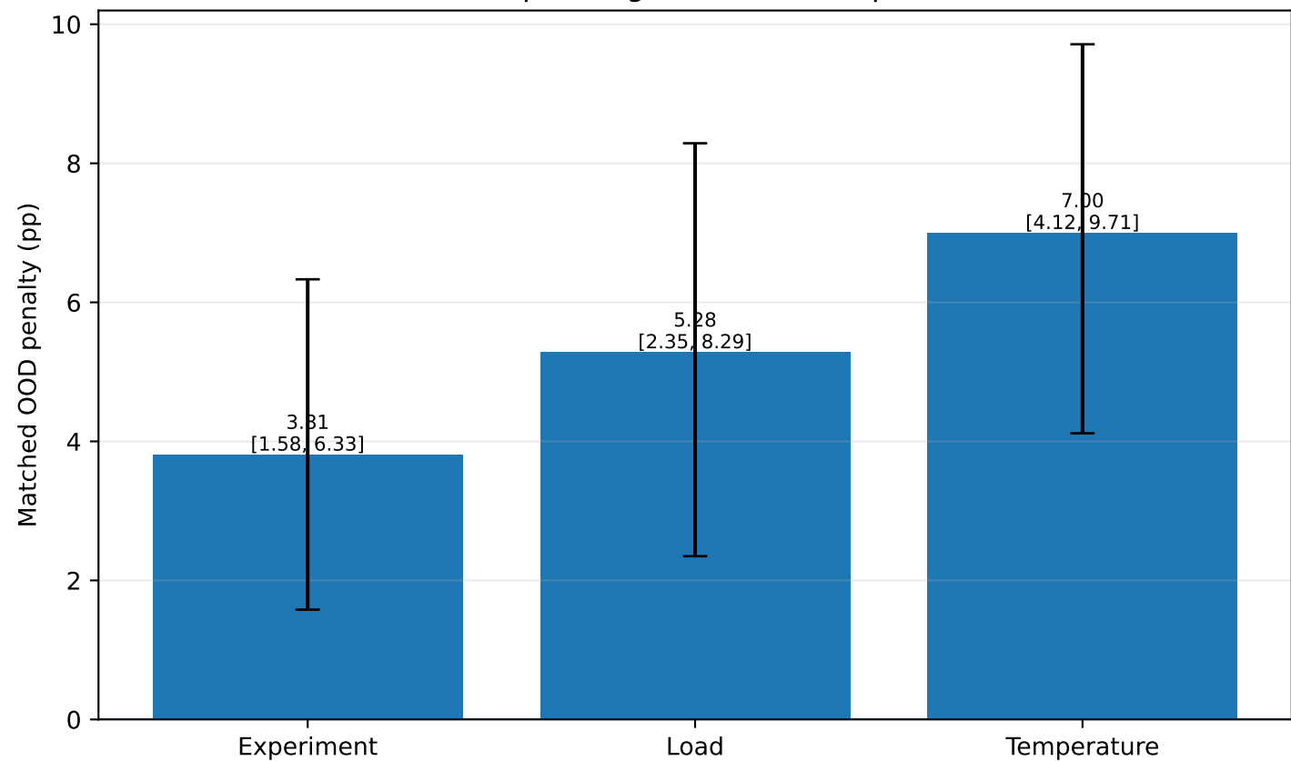
RF20x7 operating-condition shift penalties
