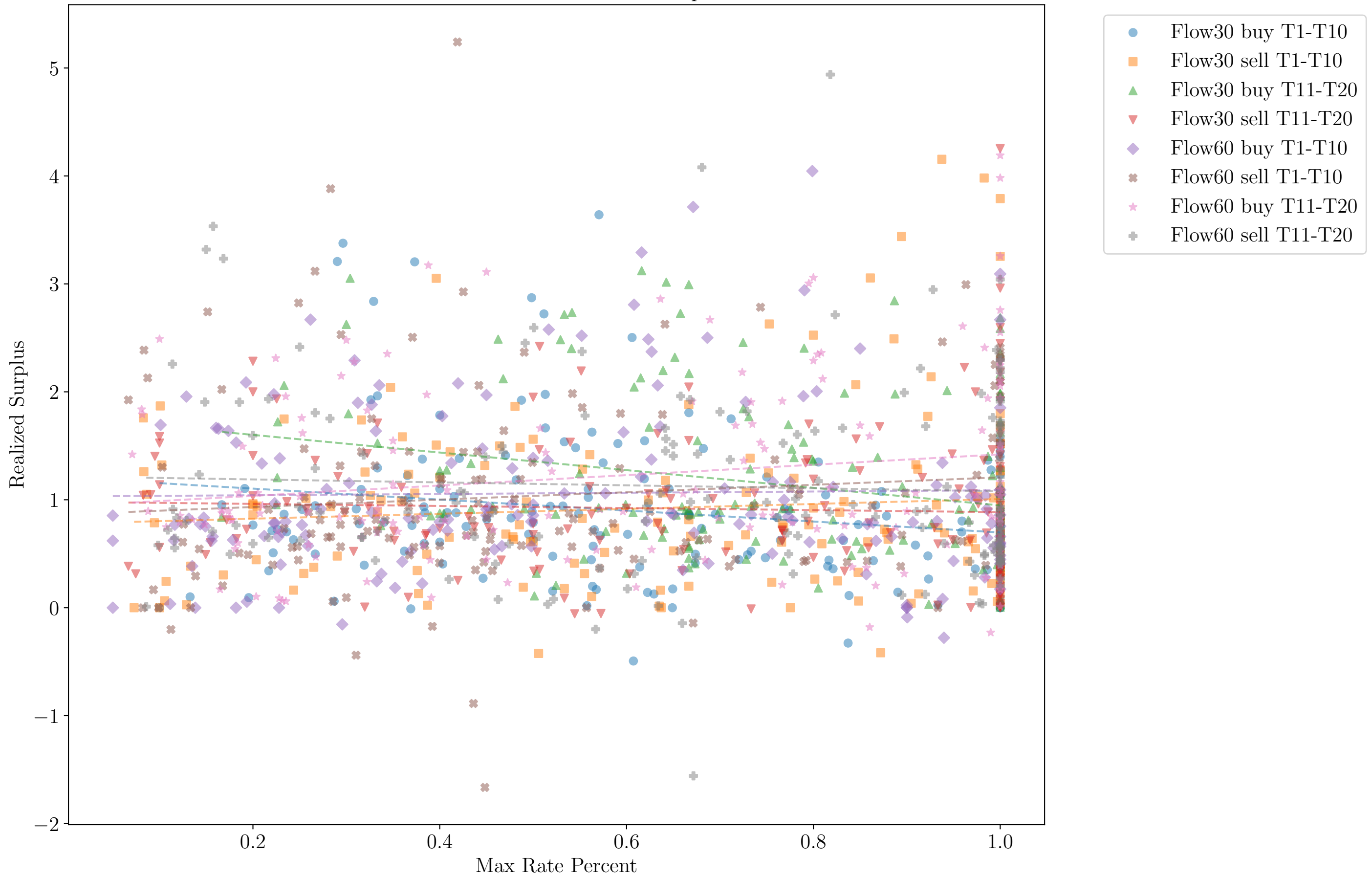
Max Rate Percent vs Realized Surplus
