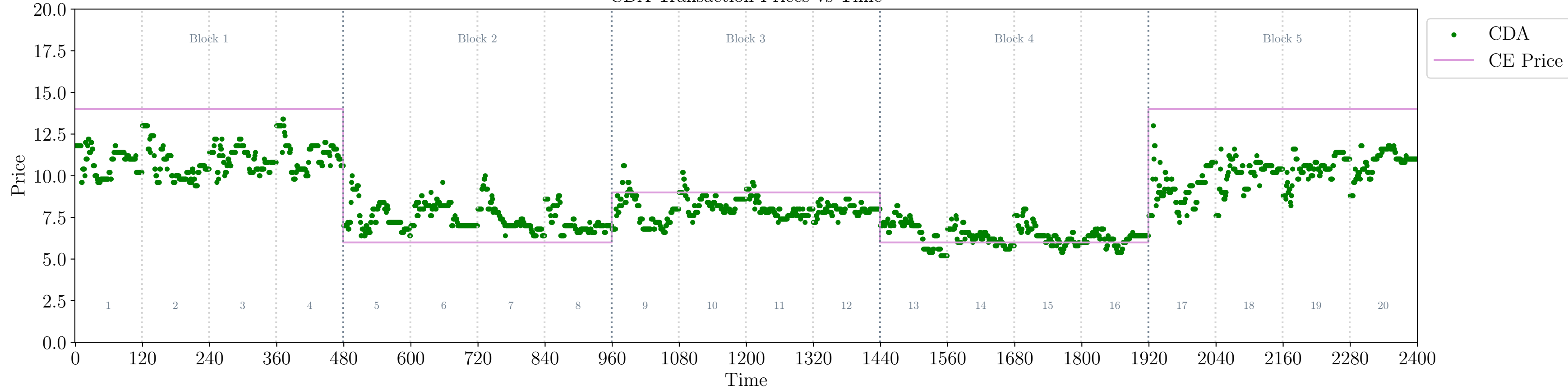
CDA Transaction Prices vs Time
