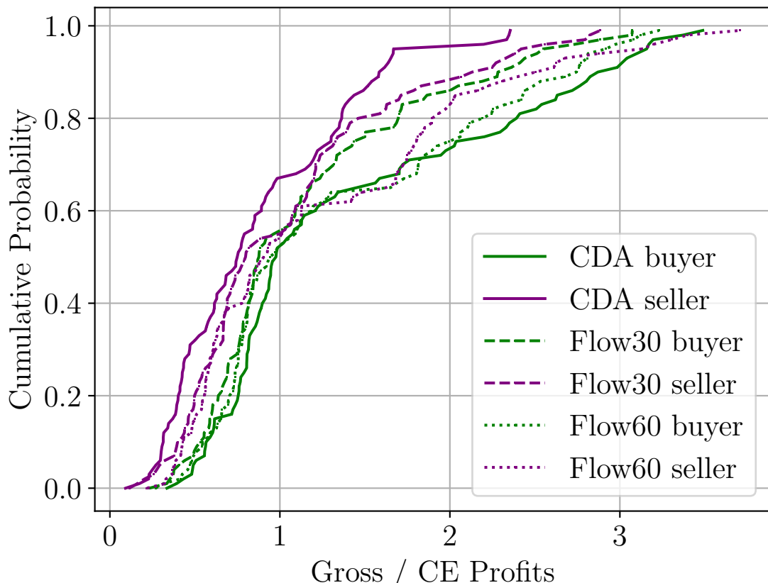
CDF of Normalized Gross Profits
