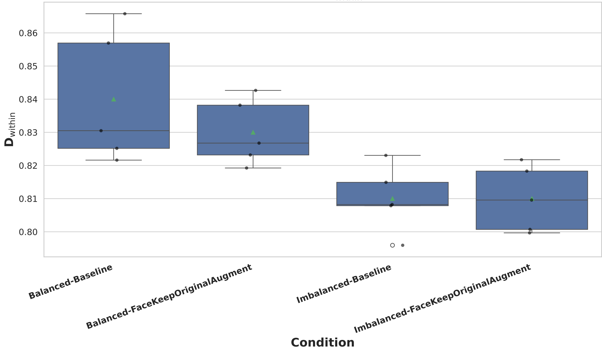
LFW: D_{\text{within}}
