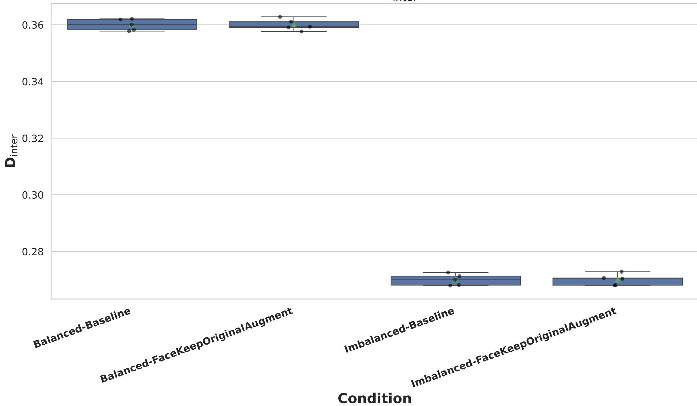
LFW: D_{\text{inter}}
