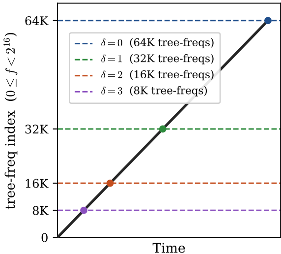
(tree-freq, time) plane
