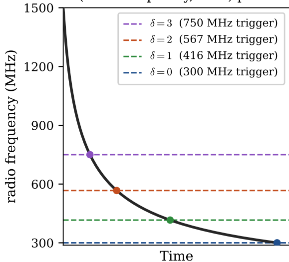
(radio-frequency, time) plane
