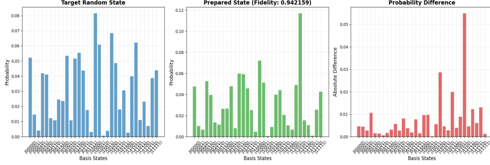
Fig. 11: Fidelity graph for Bures distance for a 5-qubit system.
