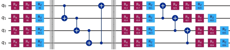
Fig. 4: Random 4-qubit ansatz architecture.
