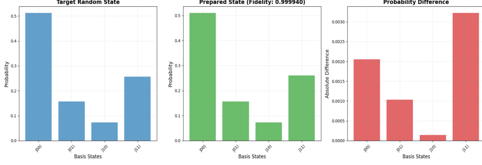
Fig. 8: Fidelity graph for Bures distance for a 2-qubit system.
