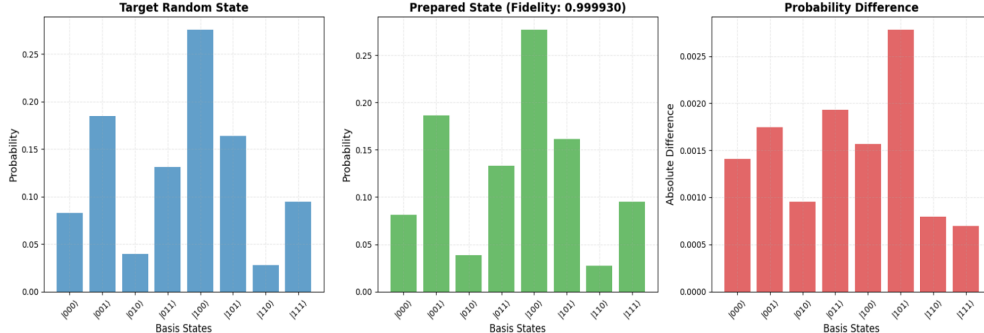
Fig. 9: Fidelity graph for Bures distance for a 3-qubit system.
