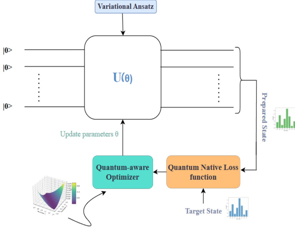
Fig. 1: Workflow methodology.
