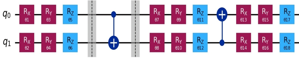
Fig. 2: Random 2-qubit ansatz architecture.
