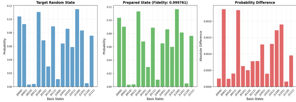
Fig. 10: Fidelity graph for Fubini Study distance for a 4-qubit system.
