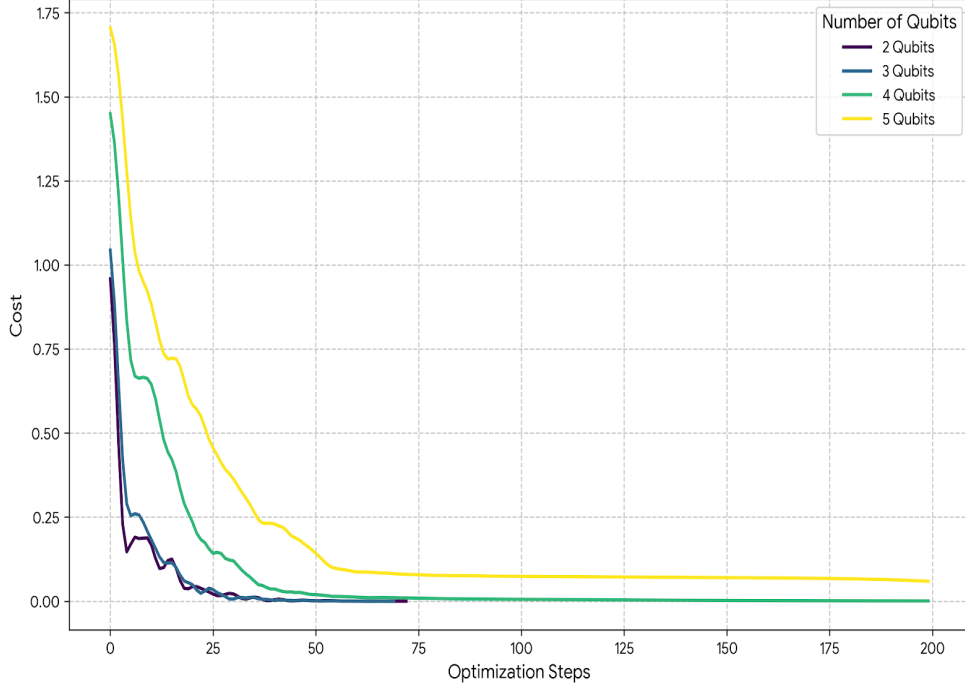
Fig. 6: Cost graph for Bures distance .
