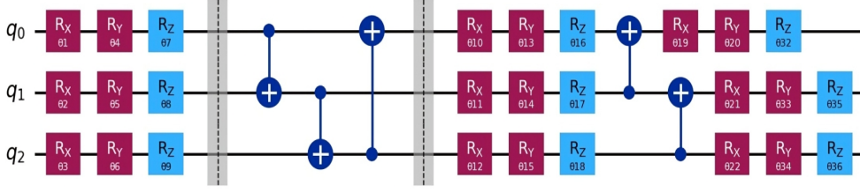
Fig. 3: Random 3-qubit ansatz architecture.
