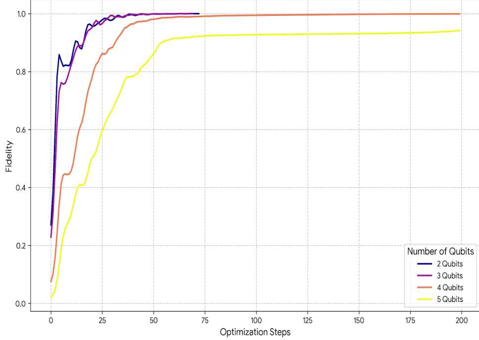
Fig. 7: Fidelity graph for Bures distance .
