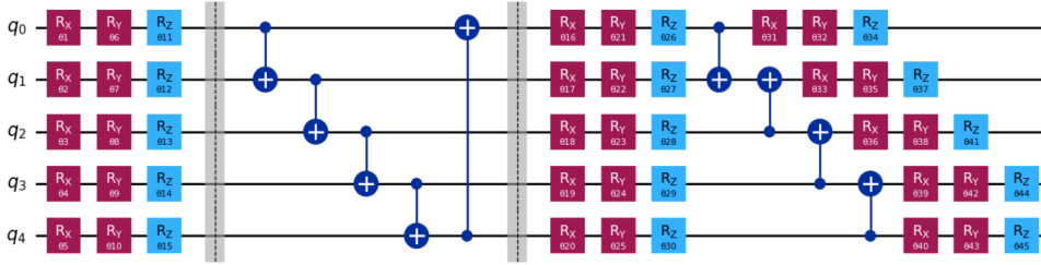
Fig. 5: Random 5-qubit ansatz architecture.
