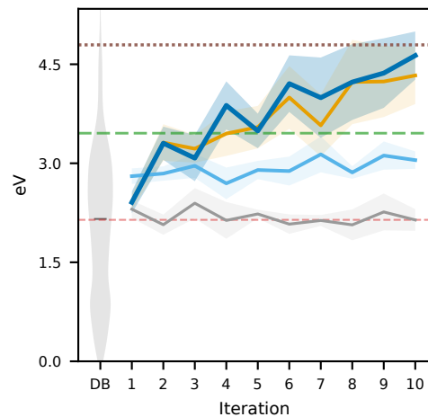
(e) Band gap > 4 eV
