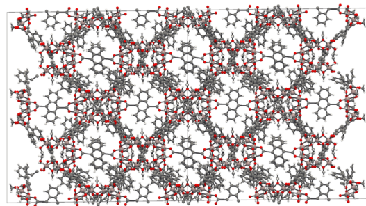
(f) Final MOF structure (H 2 , 160 K, 5 bar)
