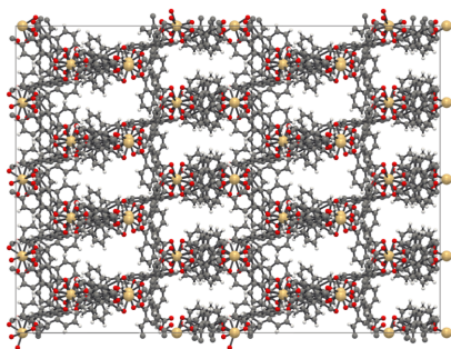
(e) Final MOF structure (H 2 , 77 K, 5 bar)
