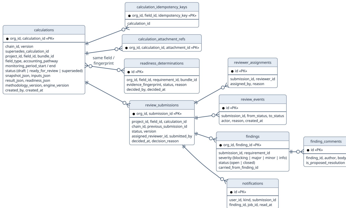
Fig 31: Calculation and internal-review persistence tables.
