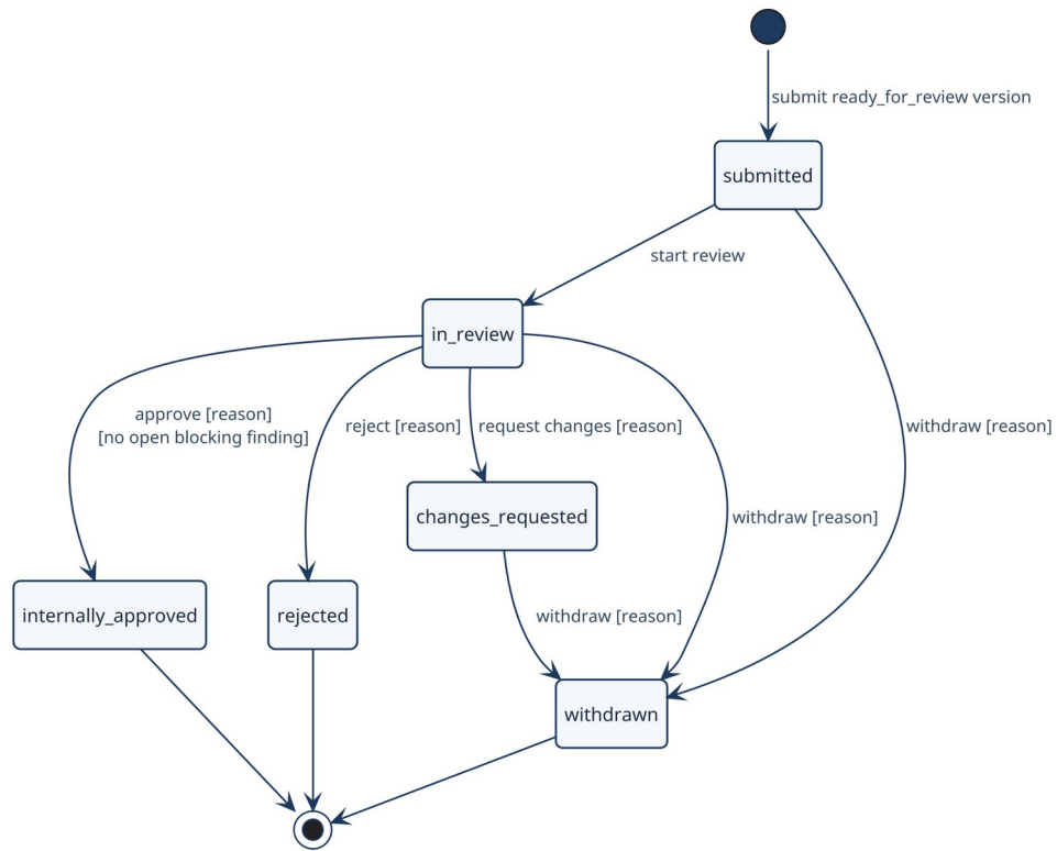
Fig 19: State diagram — internal review submission lifecycle ( src/projects/reviews.py ).
