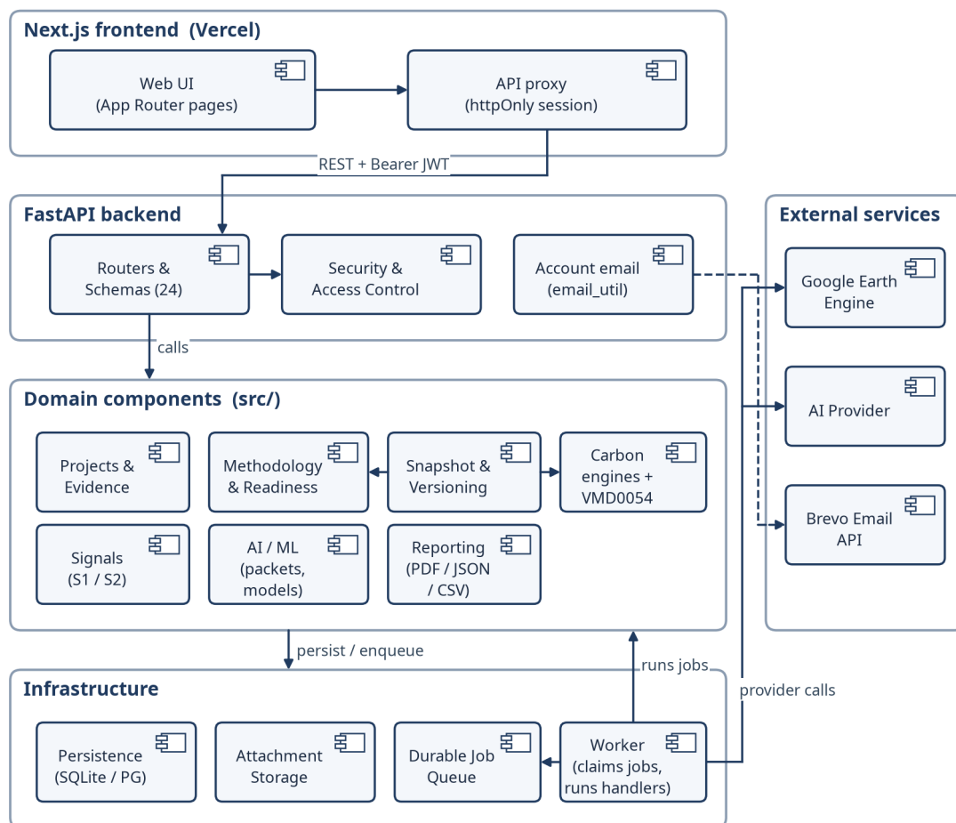
Fig 14: Top-level component diagram of Terra-Audit.
