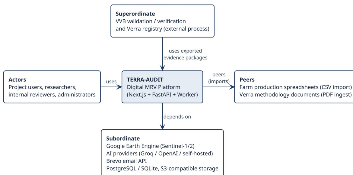
Fig 11: Architectural context diagram (ACD) of Terra-Audit.
