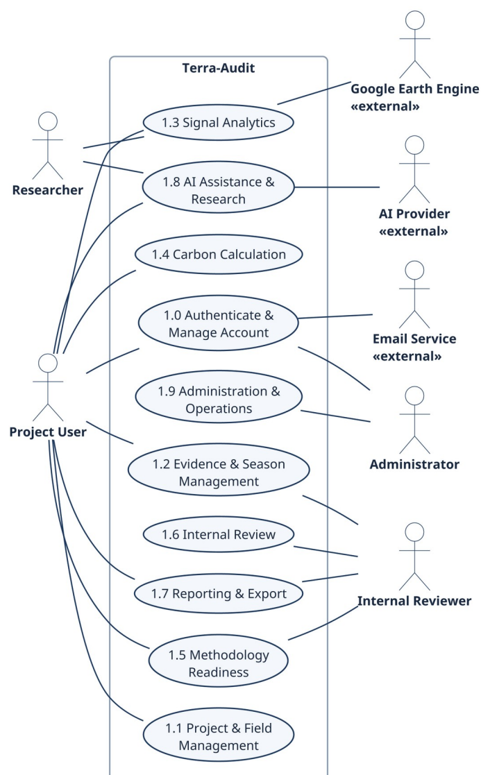
Fig 3: Use Case Level 1 — the ten user-goal modules and their actors.
