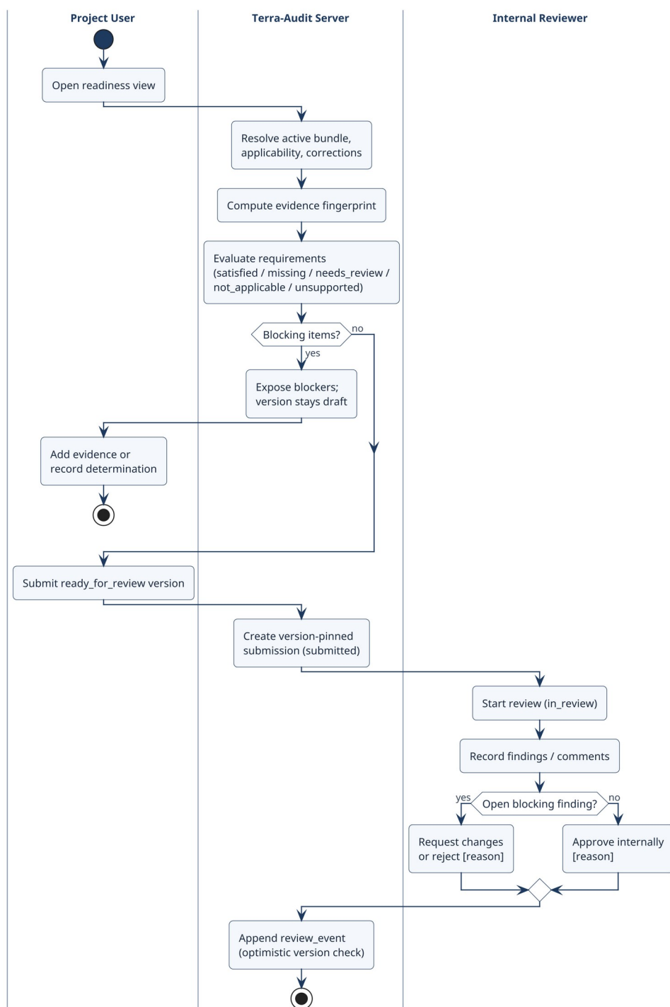
Fig 7: Activity diagram — methodology readiness and internal review with swimlanes.
