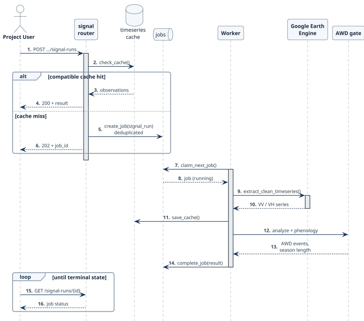
Fig 22: Sequence diagram — Sentinel-1 signal run through the durable job queue.
