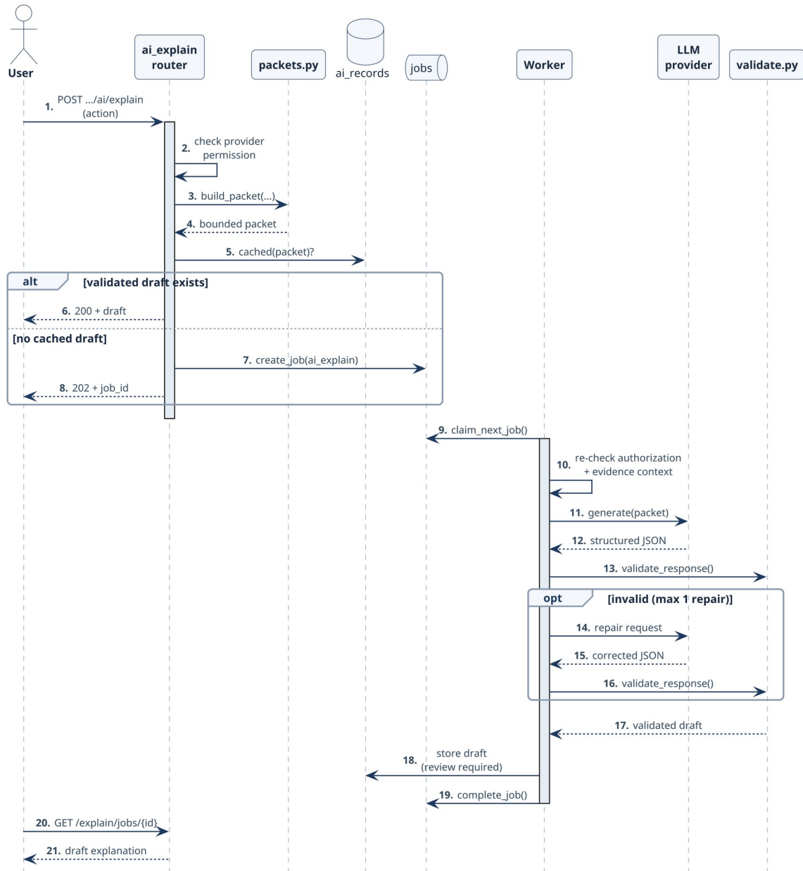
Fig 23: Sequence diagram — bounded AI explanation with server-side validation.
