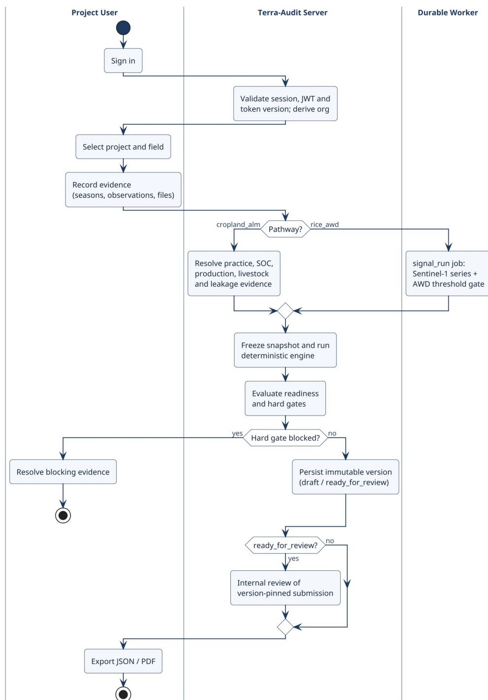
Fig 5: Overall activity diagram with swimlanes for the project user, the Terra-Audit server and the durable worker.
