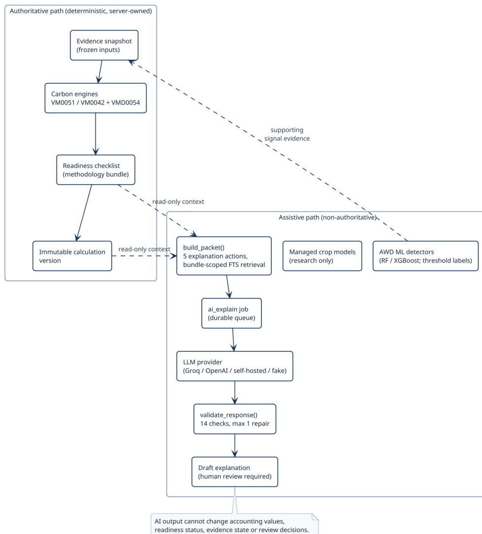
Fig 25: AI authority and data flow: deterministic, server-owned accounting path versus the non-authoritative assistive path.
