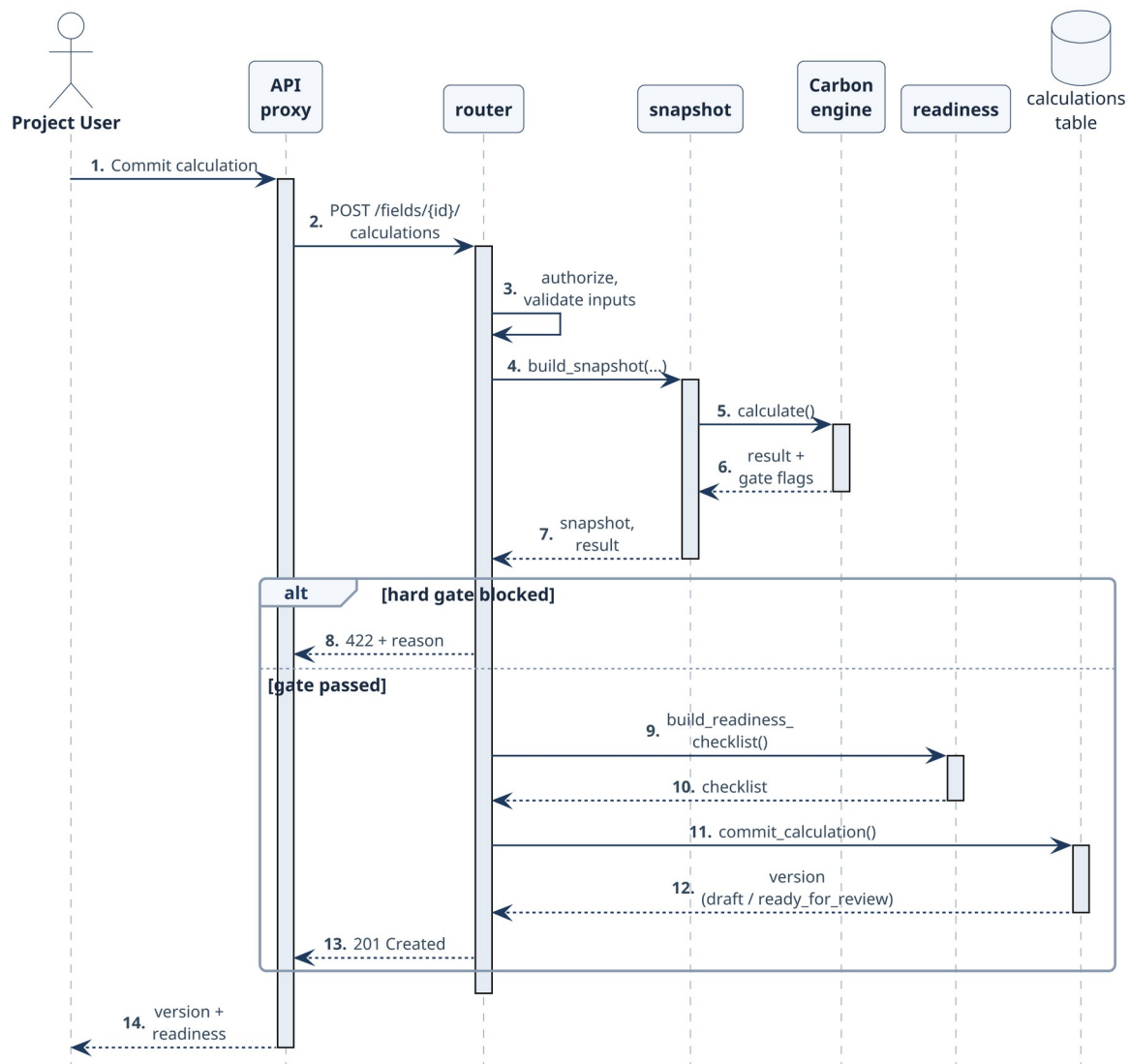
Fig 20: Sequence diagram — calculation commit from authenticated request to immutable version.
