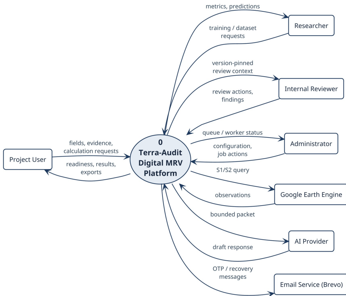
Fig 15: Level-0 data-flow diagram: external entities and the information they exchange with Terra-Audit.
