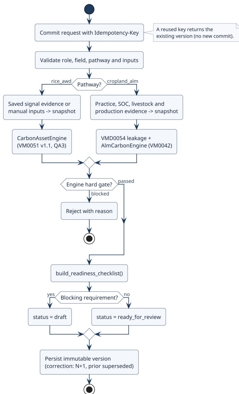
Fig 6: Activity diagram — versioned carbon calculation commit.
