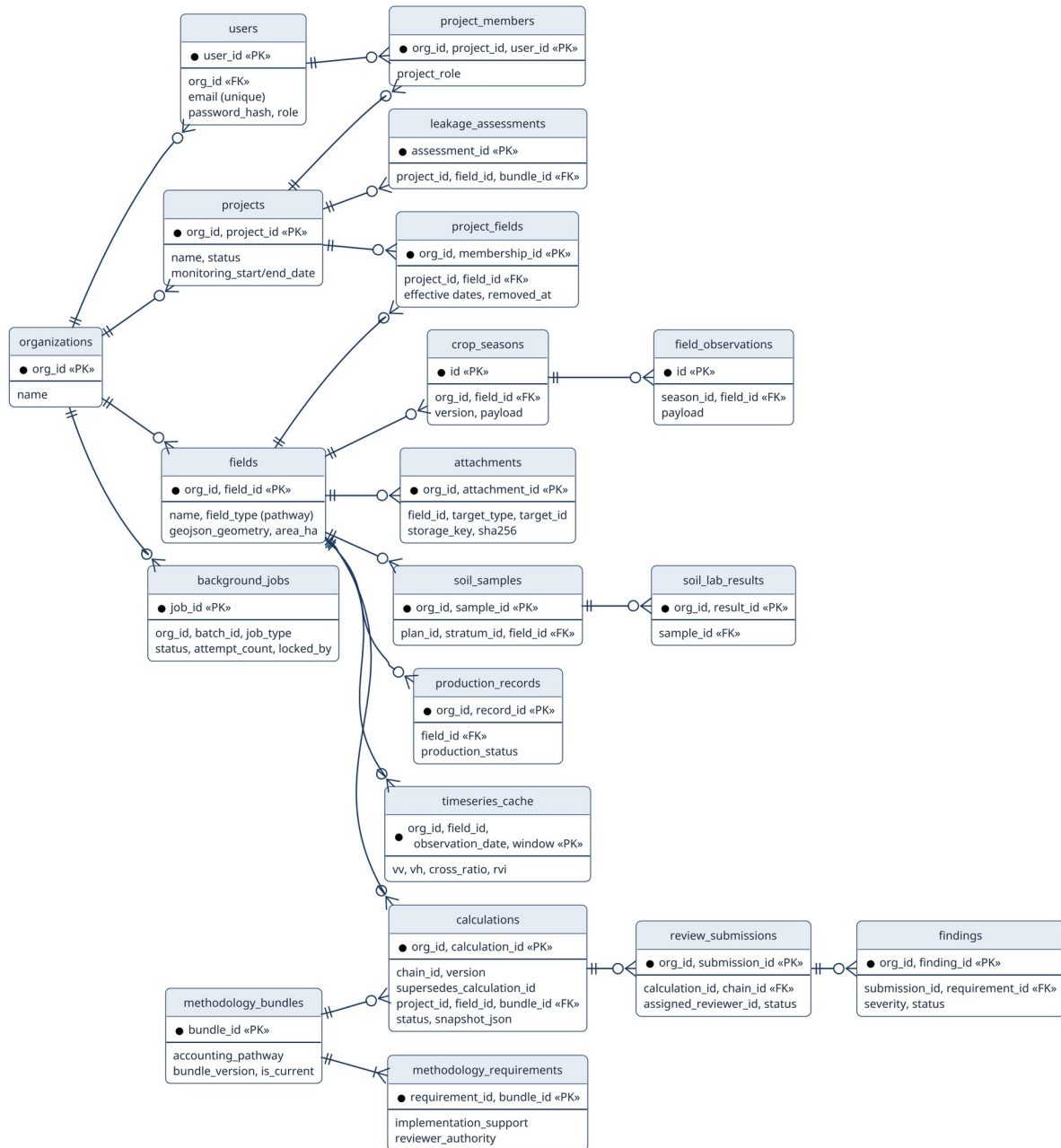
Fig 8: Entity-relationship diagram (crow's-foot notation) of the core persistent entities.
