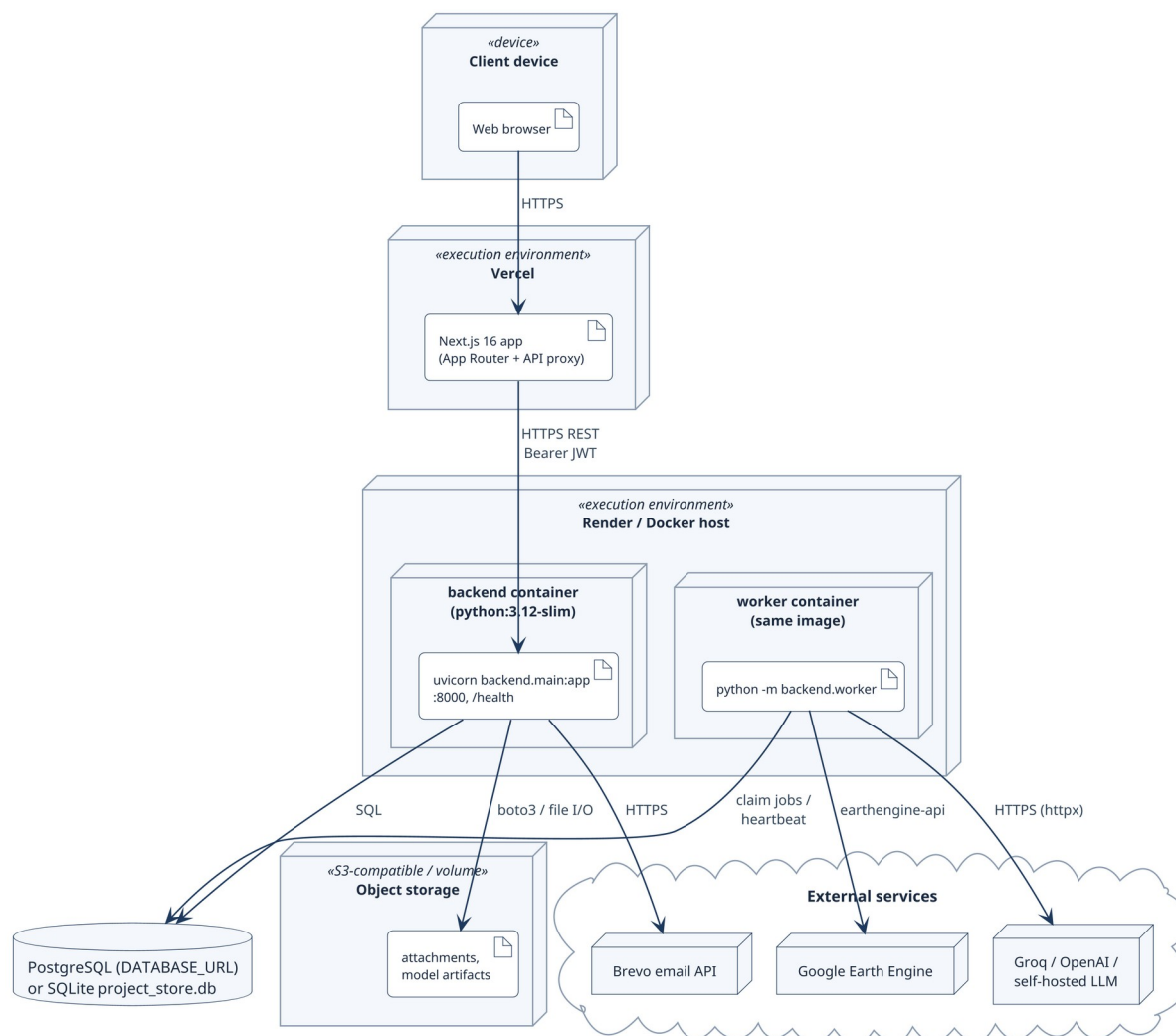
Fig 24: UML deployment diagram of Terra-Audit.
