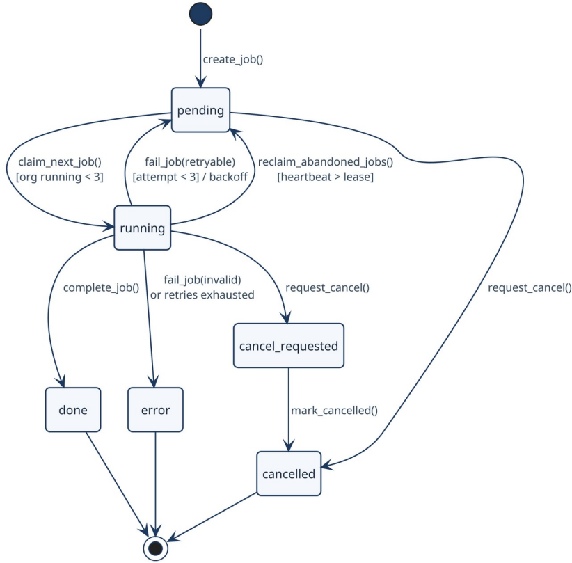
Fig 17: State diagram — durable background job lifecycle (src/jobs/queue.py).
