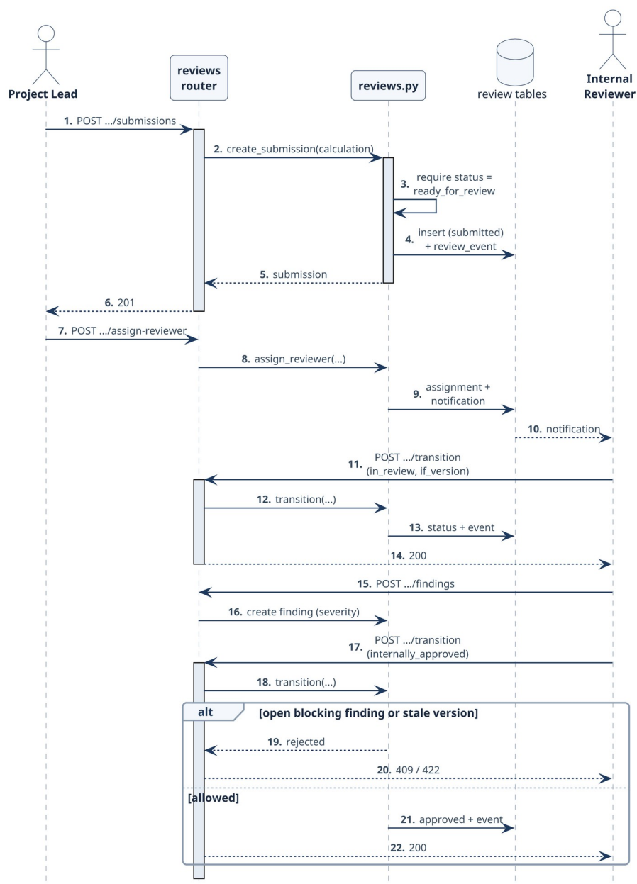
Fig 21: Sequence diagram — internal review from submission to guarded decision.
