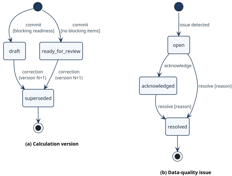
Fig 18: State diagrams — (a) calculation version lifecycle and (b) data-quality issue lifecycle.
