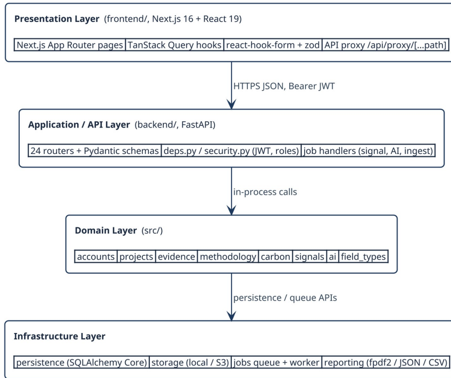
Fig 12: Layered architecture archetype instantiated for Terra-Audit.
