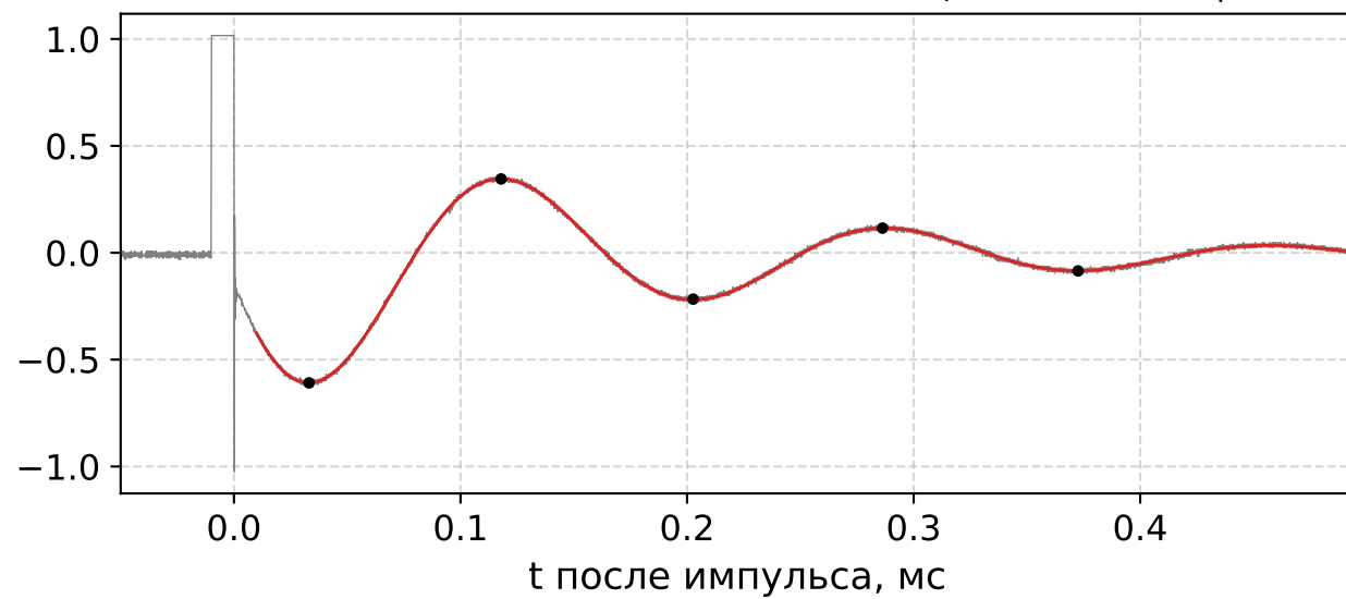
R = 1750 Ом: \Theta = 1.512 \pm 0.007 , f = 5818 Гц
