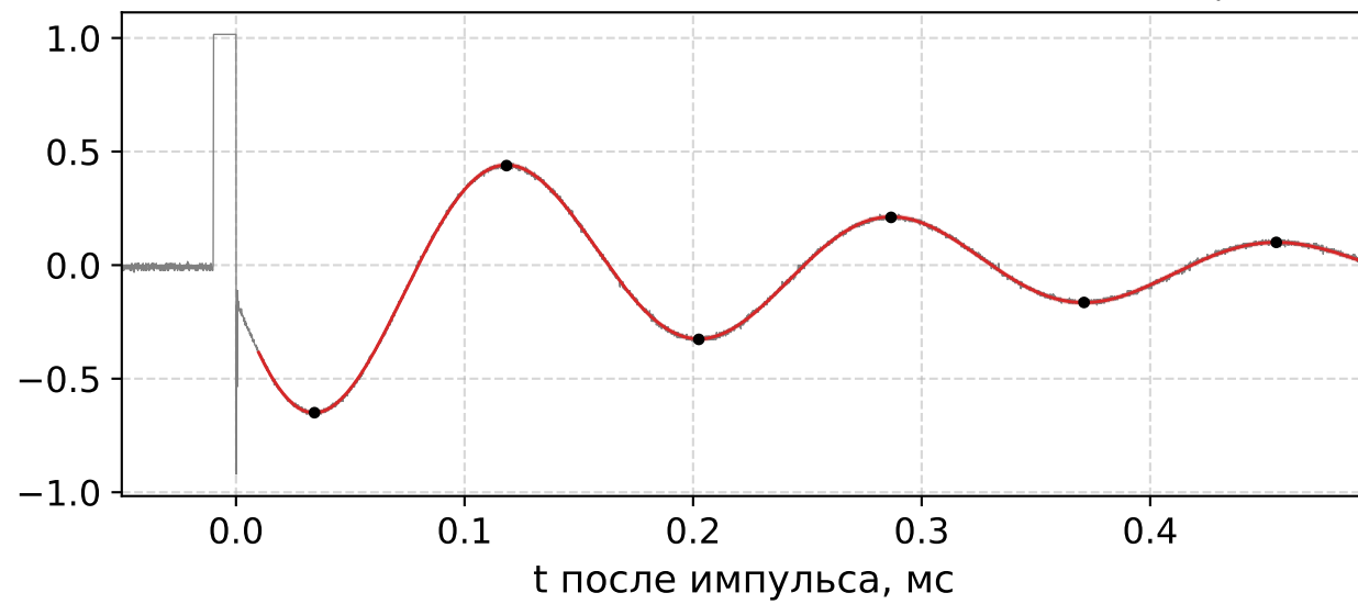
R = 1200 Ом: \Theta = 1.042 \pm 0.002 , f = 5899 Гц
