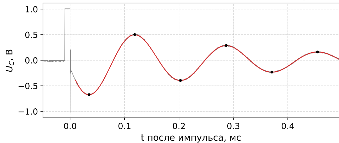
R = 1000 Ом: \Theta = 0.873 \pm 0.004 , f = 5919 Гц
