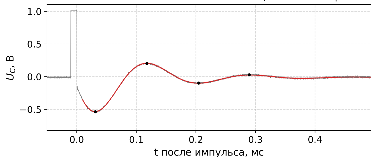
R = 2040 Ом: \Theta = 1.778 \pm 0.020 , f = 5767 Гц
