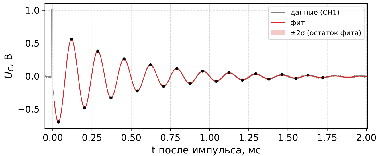
R = 800 Ом: \Theta = 0.707 \pm 0.001 , f = 5938 Гц
