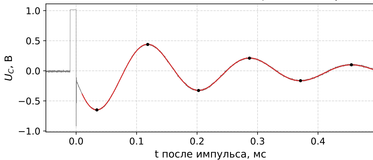
R = 1200 Ом: \Theta = 1.042 \pm 0.002 , f = 5899 Гц
