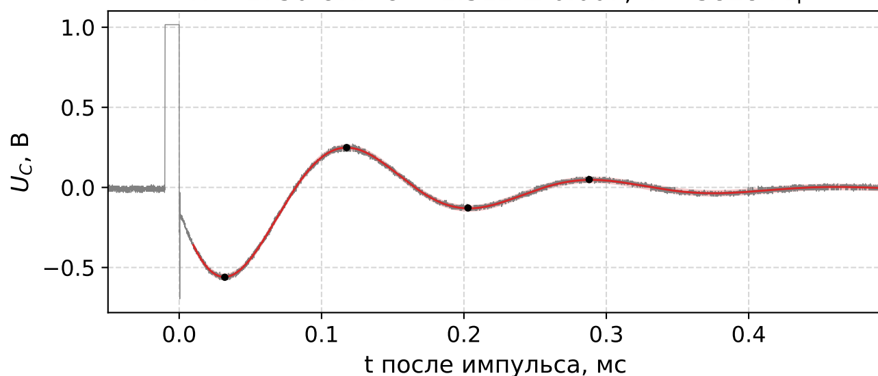
R = 1750 Ом: \Theta = 1.512 \pm 0.007 , f = 5818 Гц
