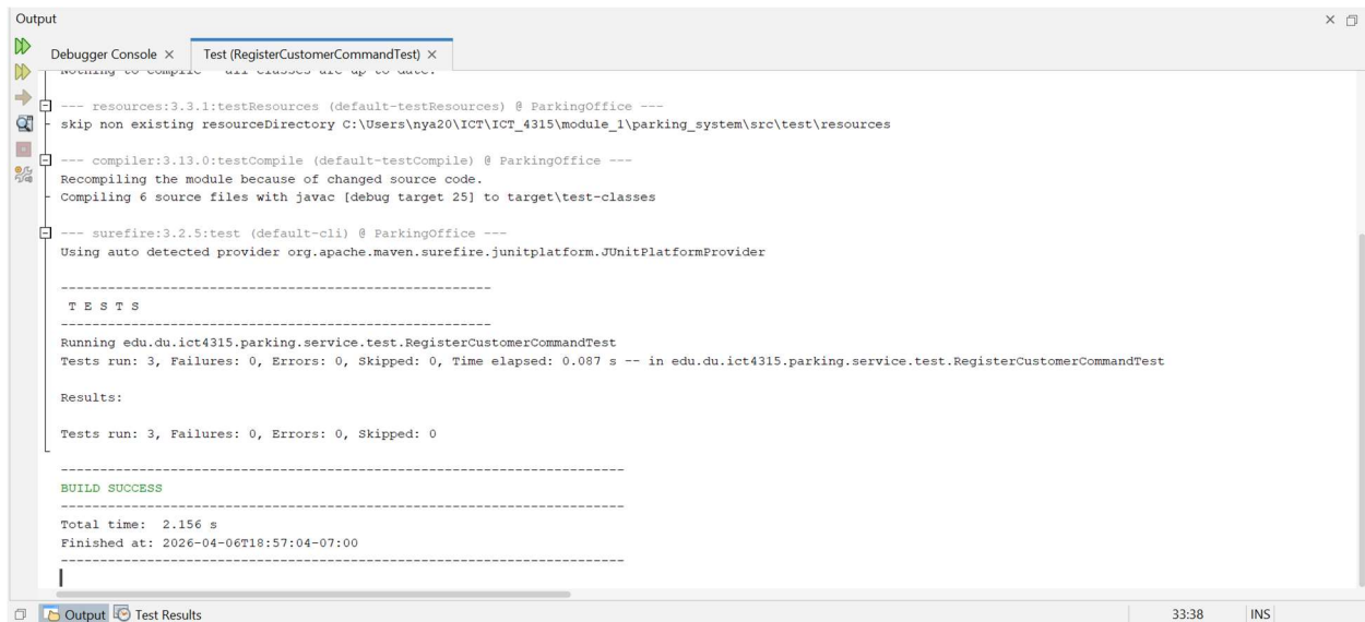
Figure 1. JUnit test results for RegisterCustomerCommandTest
