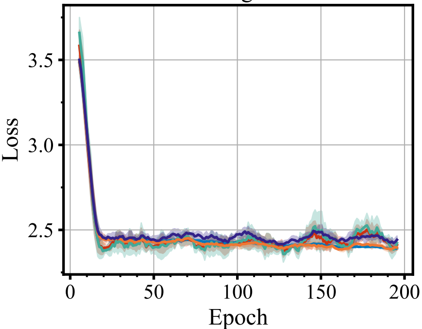
Training Loss
