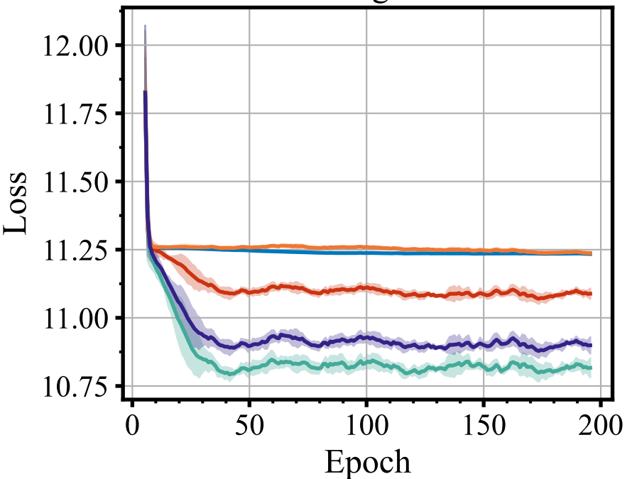
Training Loss
