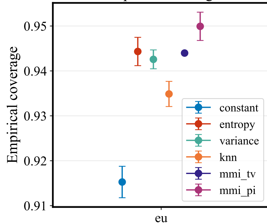
Empirical coverage
