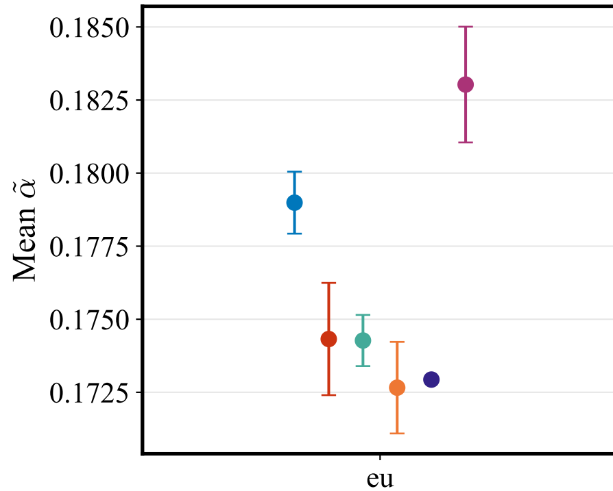
Mean \tilde{\alpha}
