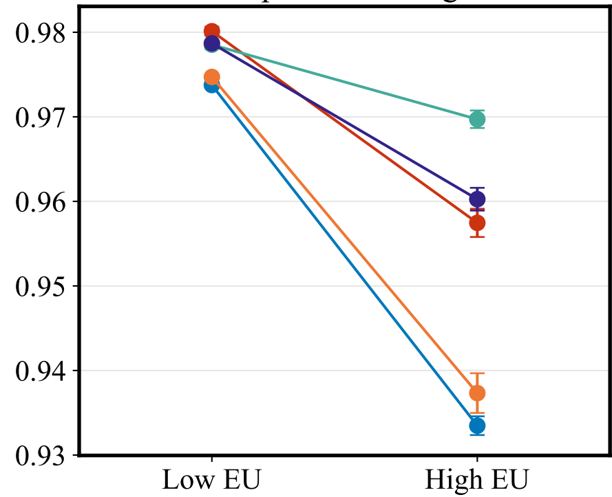
Empirical coverage
