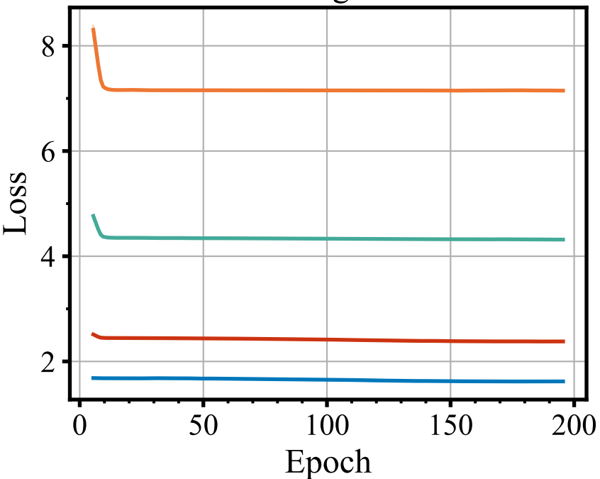
Training Loss
