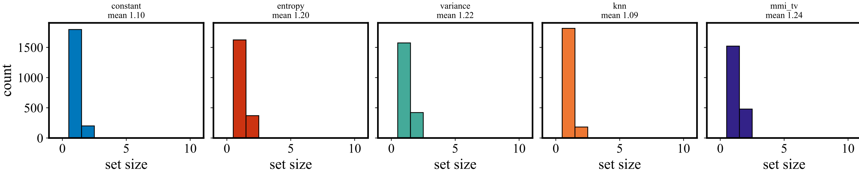
Conformal set sizes on the test split
